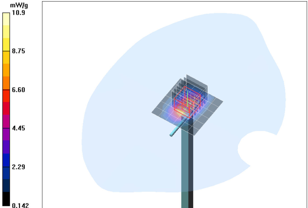
Fig. 12: Validation measurement 1900 MHz body (December 02, 2010), coarse grid. Ambient Temperature: 21.4° C, Liquid Temperature: 21.2° C.
