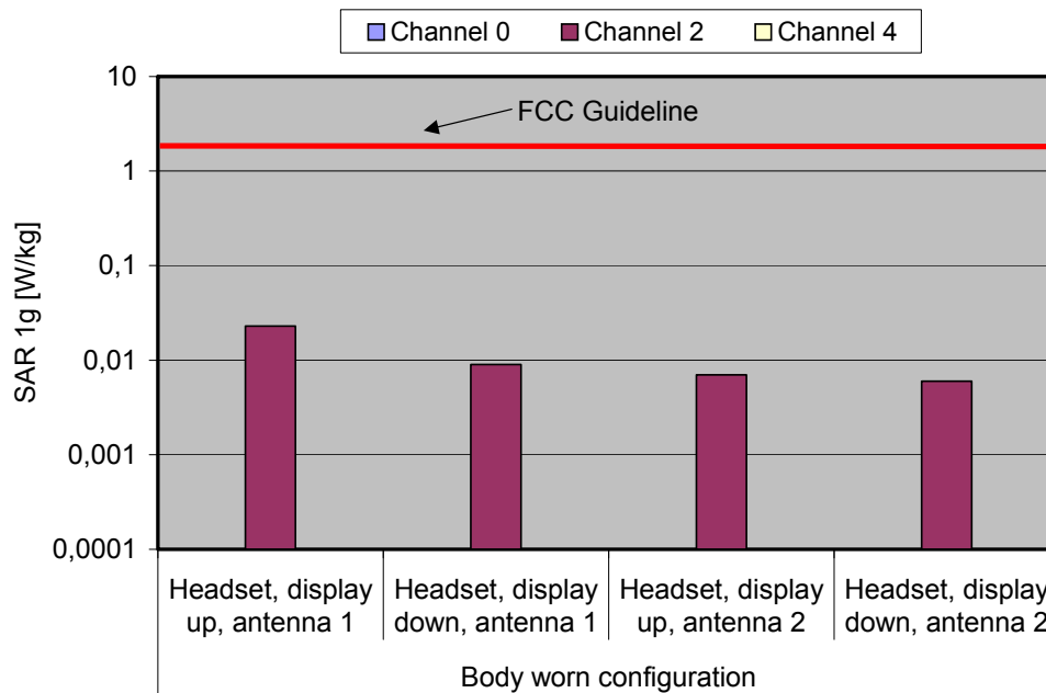
Fig. 10: The measured SAR values in body-worn configuration for the RTX RTX8660 / Uniden EXP1240H for the US DECT standard in comparison to the FCC exposure limit.
