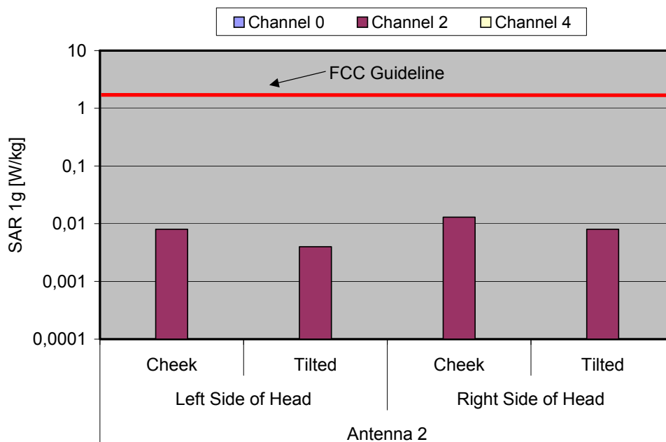
Fig. 9: The measured head phantom SAR values for the RTX RTX8660 / Uniden EXP1240H, with antenna 2 for the US DECT standard in comparison to the FCC exposure limit.
