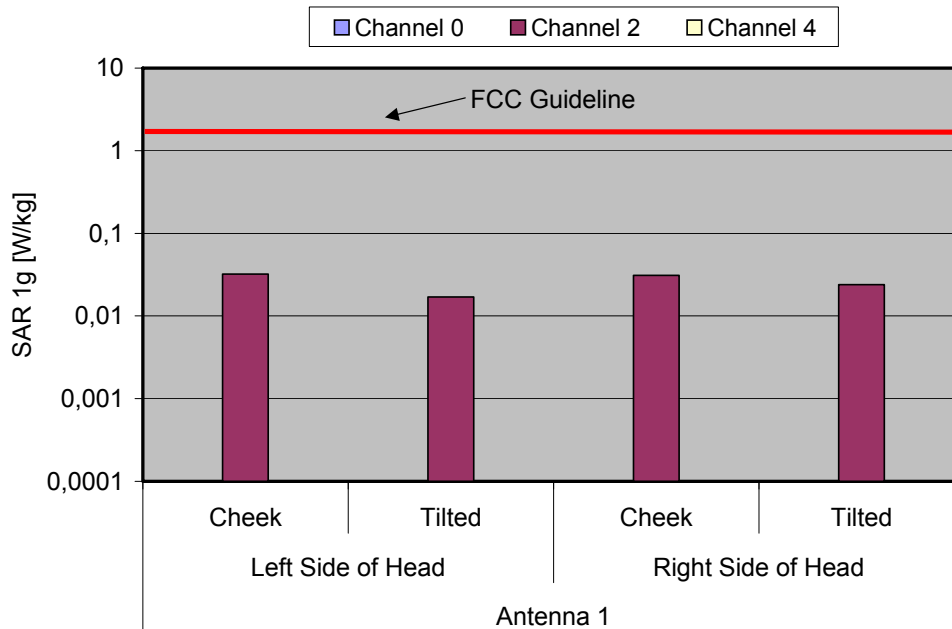
Fig. 8: The measured head phantom SAR values for the RTX RTX8660 / Uniden EXP1240H, with antenna 1 for the US DECT standard in comparison to the FCC exposure limit.
