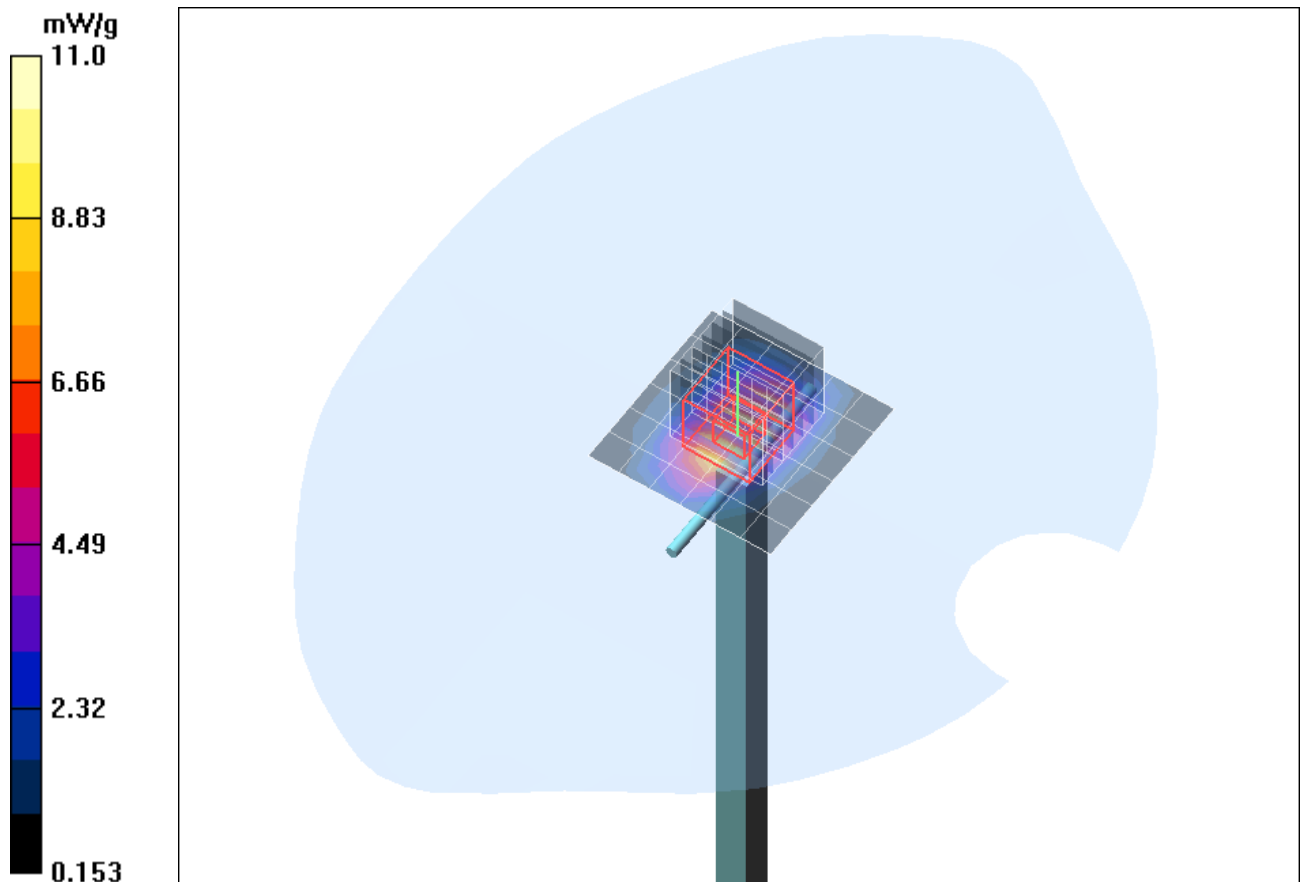
Fig. 11: Validation measurement 1900 MHz Head (December 03, 2010), coarse grid. Ambient Temperature: 21.0° C, Liquid Temperature: 20.8° C.
