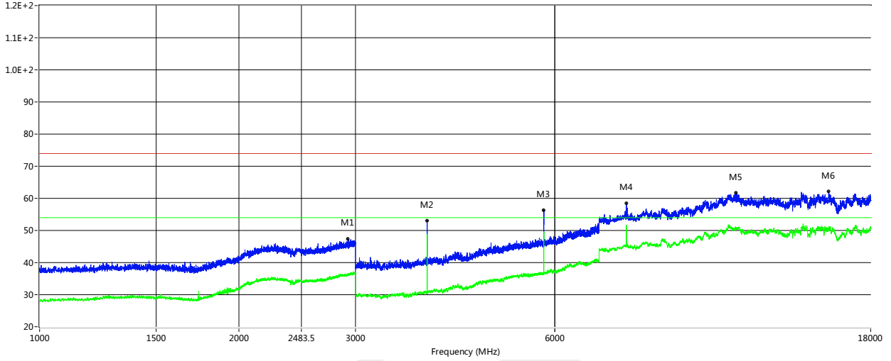
RE_FCC Test Case_FCC 15C 1GHz-18GHz
