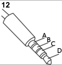
Jack connector - CTIA standards
