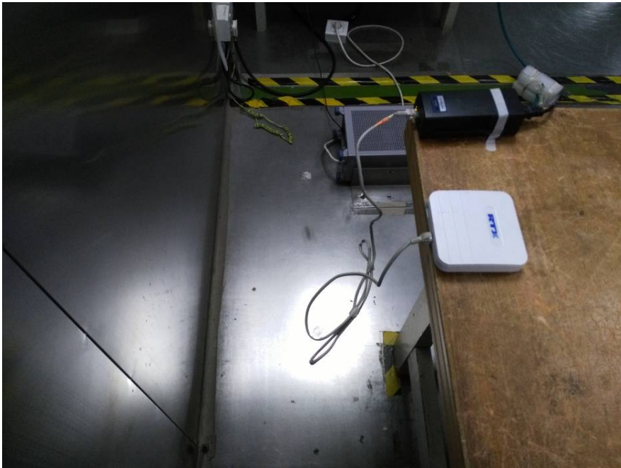
Conducted Emissions - Side View (Power by POE)
