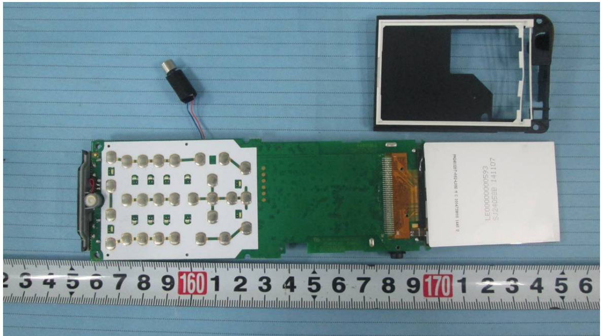
EUT –Main Board Bottom LCD off View
