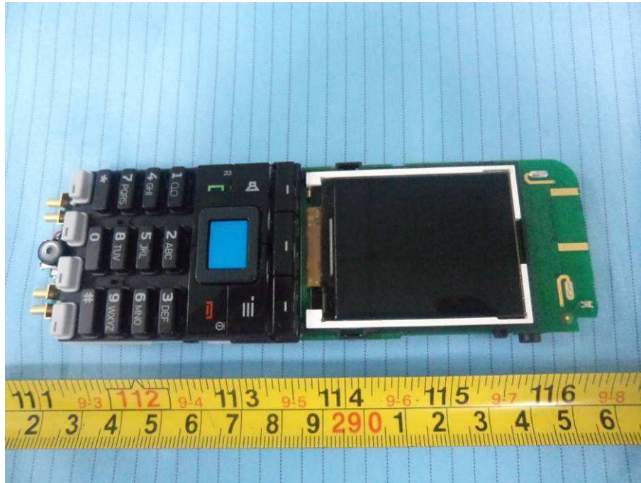
EUT – Main Board Top with Keyboard & Display View
