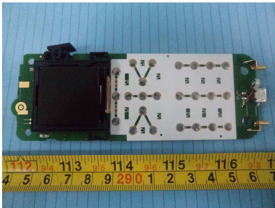
EUT – Main Board Bottom without Keyboard View
