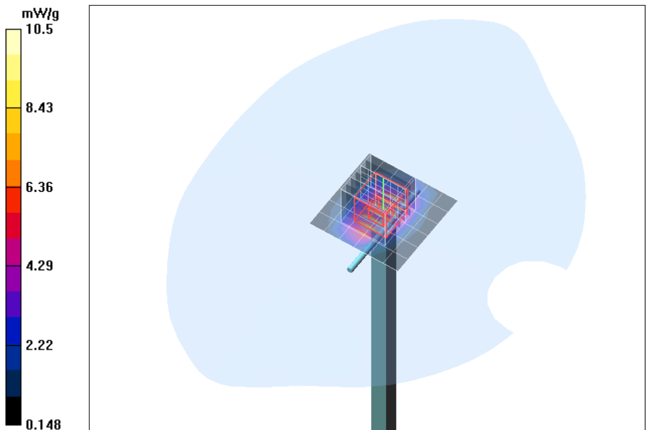
Fig. 10: Validation measurement 1900 MHz Head (January 19, 2012), coarse grid. Ambient Temperature: 21.5° C, Liquid Temperature: 21.3° C.
