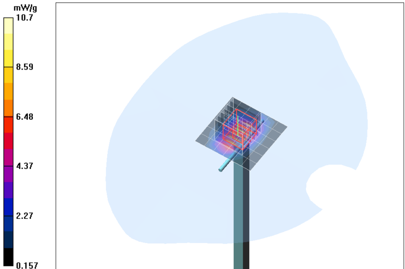
Fig. 11: Validation measurement 1900 MHz body (January 17, 2012), coarse grid. Ambient Temperature: 21.3° C, Liquid Temperature: 21.1° C.
