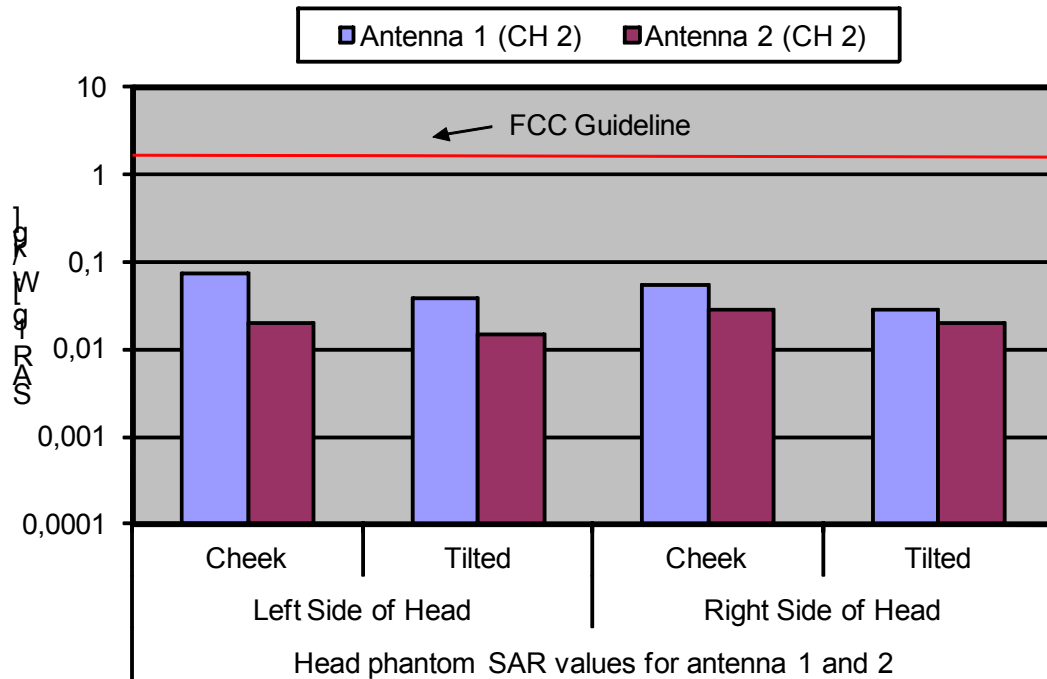
Fig. 8: The measured head phantom SAR values for the RTX Products RTX8111 for the US DECT standard in comparison to the FCC exposure limit.
