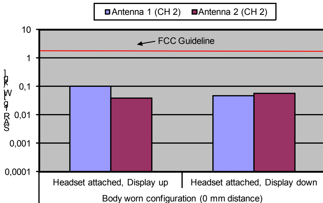
Fig. 9: The measured SAR values in body worn configuration for the RTX Products RTX8111 for the US DECT standard in comparison to the FCC exposure limit.
