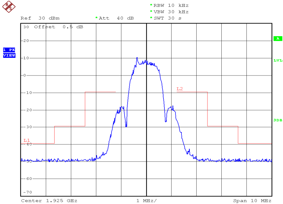
Communicator unit, Middle channel, Traffic carrier
