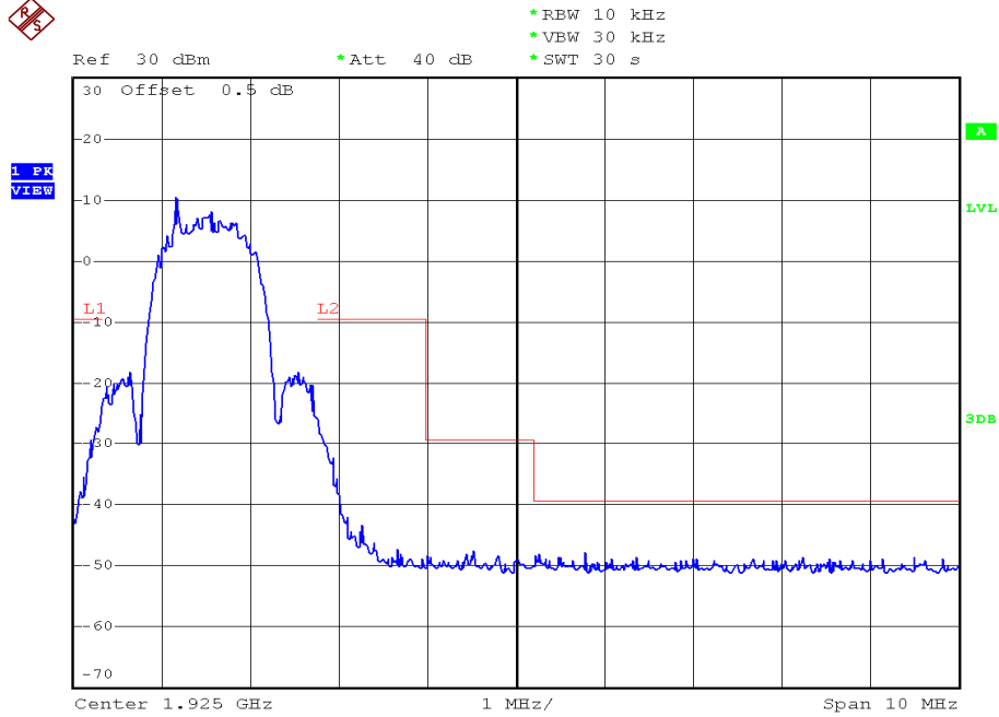
Communicator unit, Lowest channel, Traffic carrier
