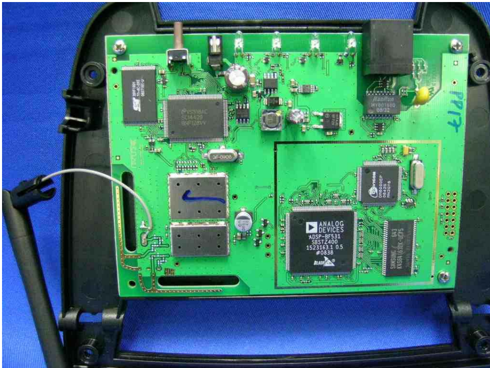
VoIP Gateway Main PCB comp side
