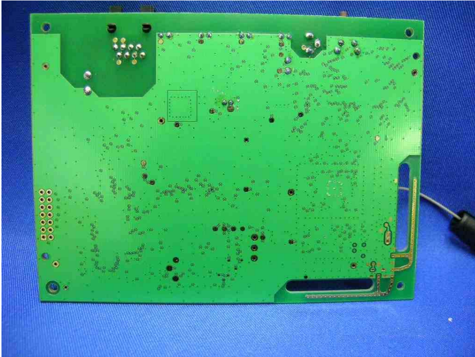
VoIP Gateway Main PCB solder side
