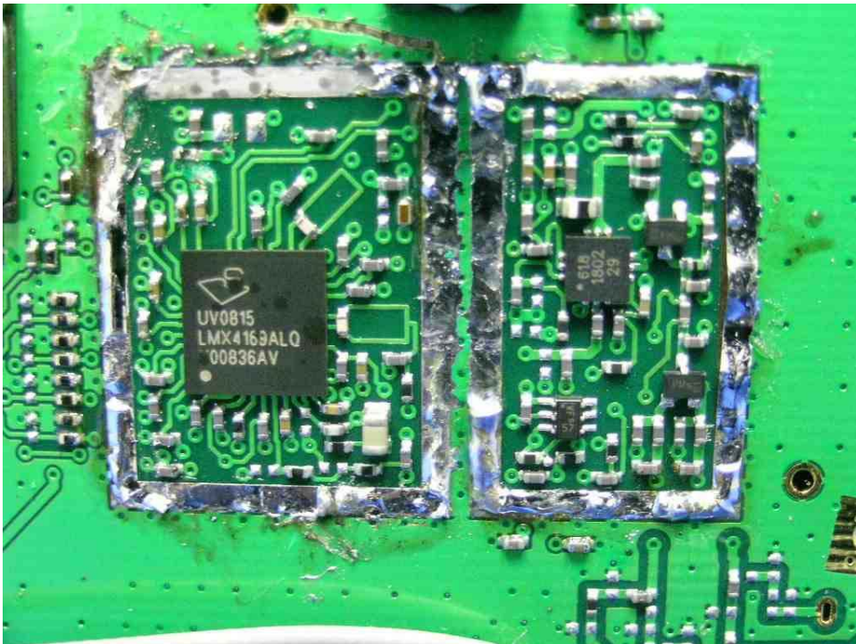
VoIP Gateway Oscillator PCB comp side
