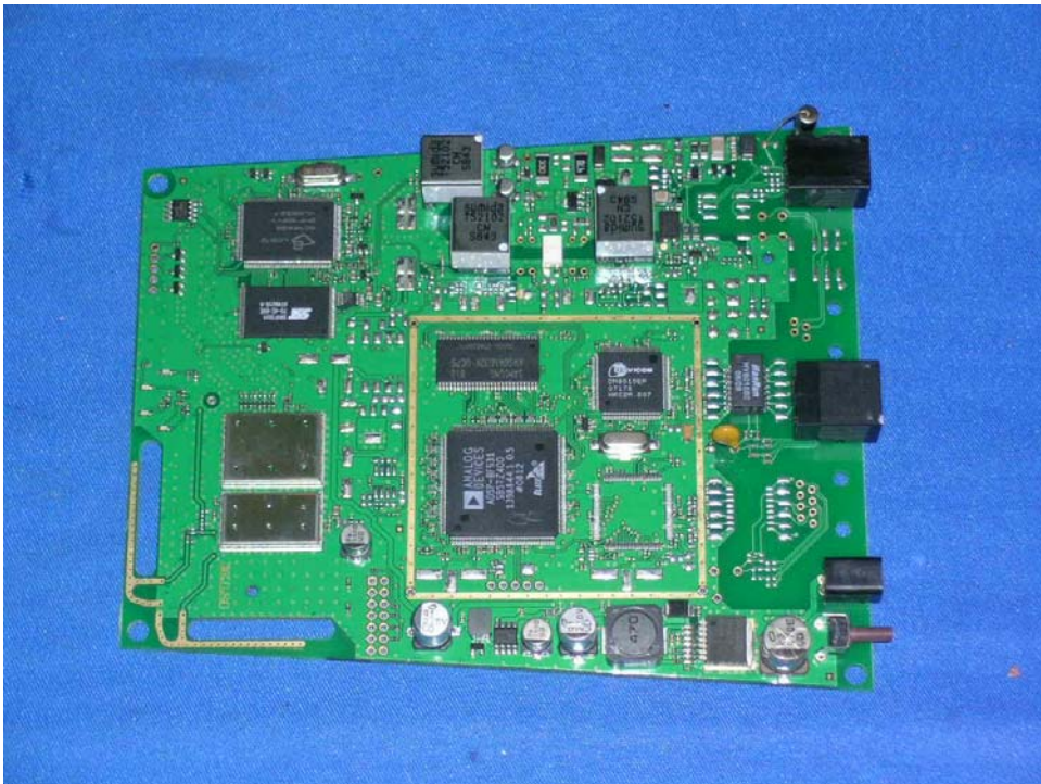
VoIP and PSTN Gateway Main PCB comp side
