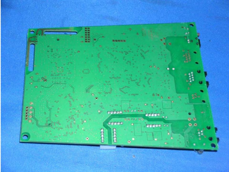
VoIP and PSTN Gateway Main PCB solder side
