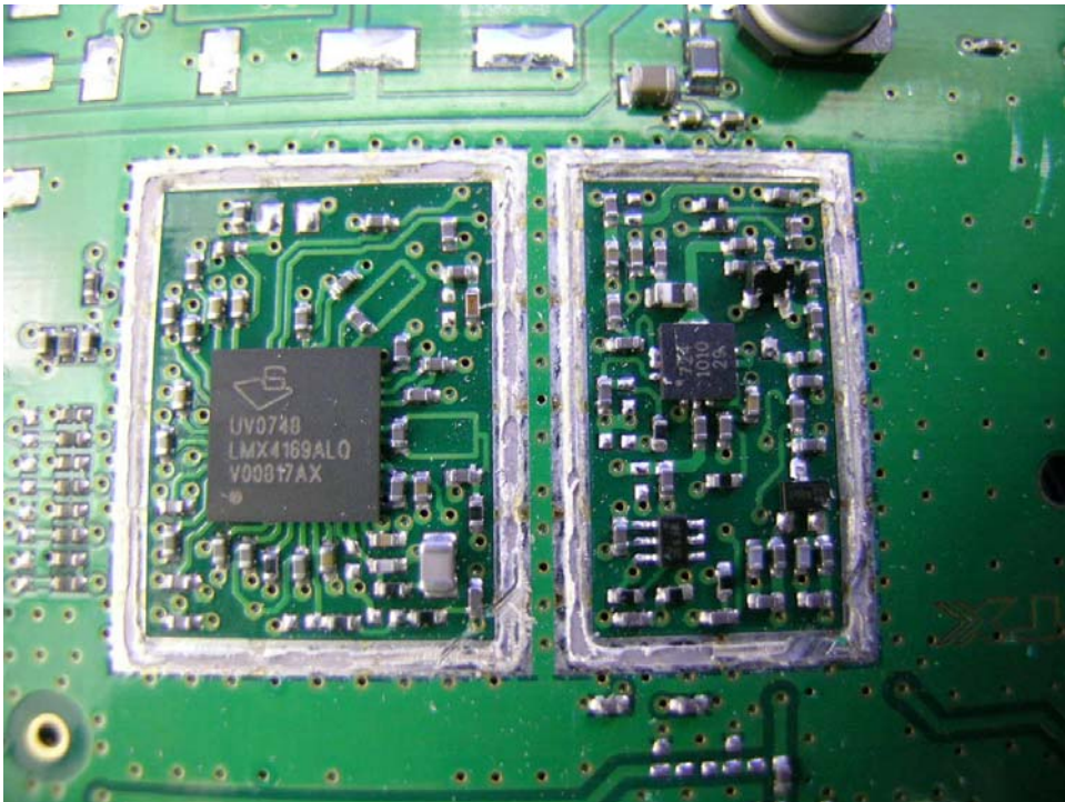
VoIP and PSTN Gateway Oscillator PCB comp side
