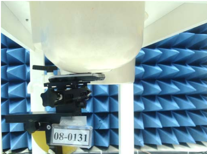
Figure 16. Left Head SAR Test Setup (Cheek)
