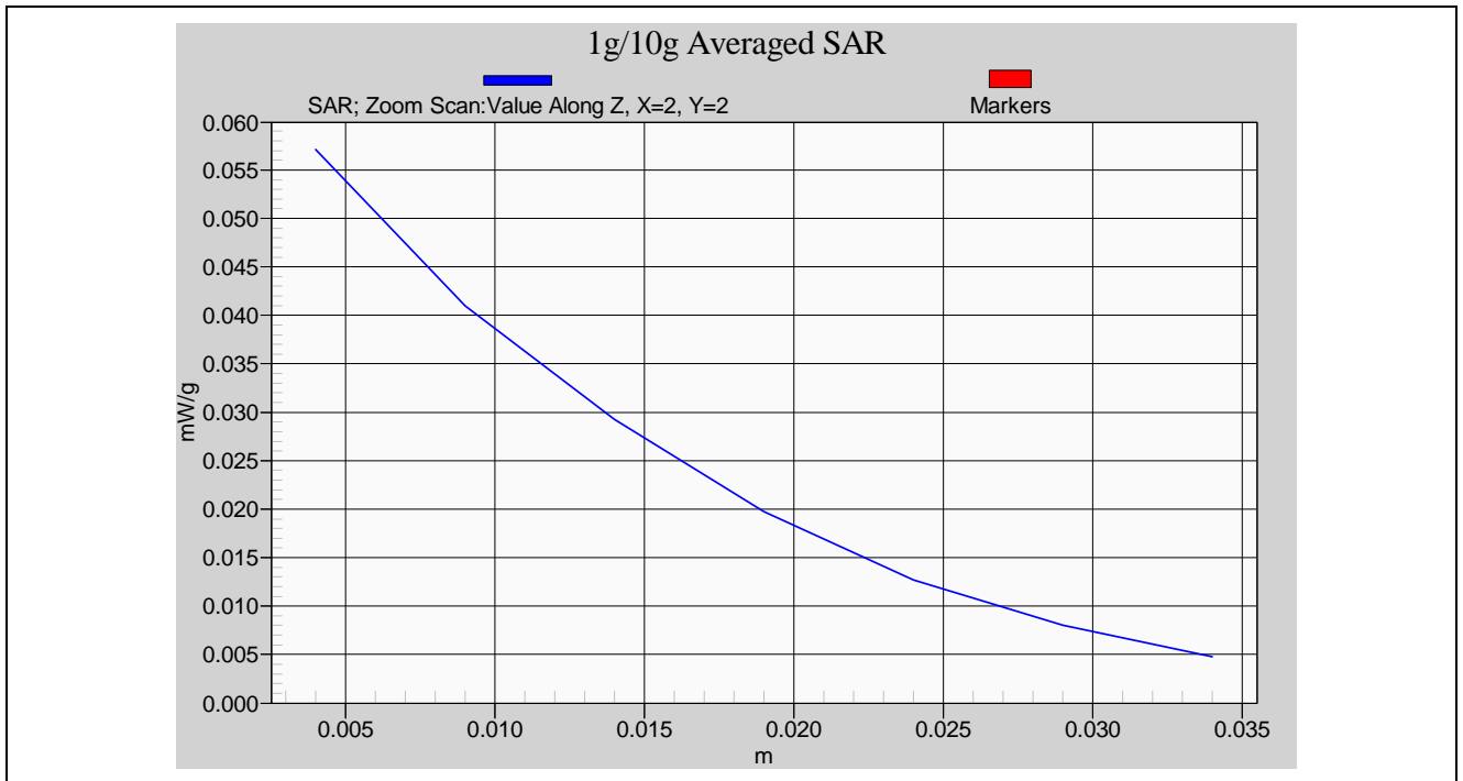
Body SAR Measurement _ CH0
