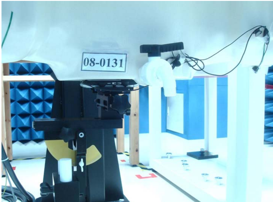
Figure 18. Body SAR Test Setup _ Back to Phantom
