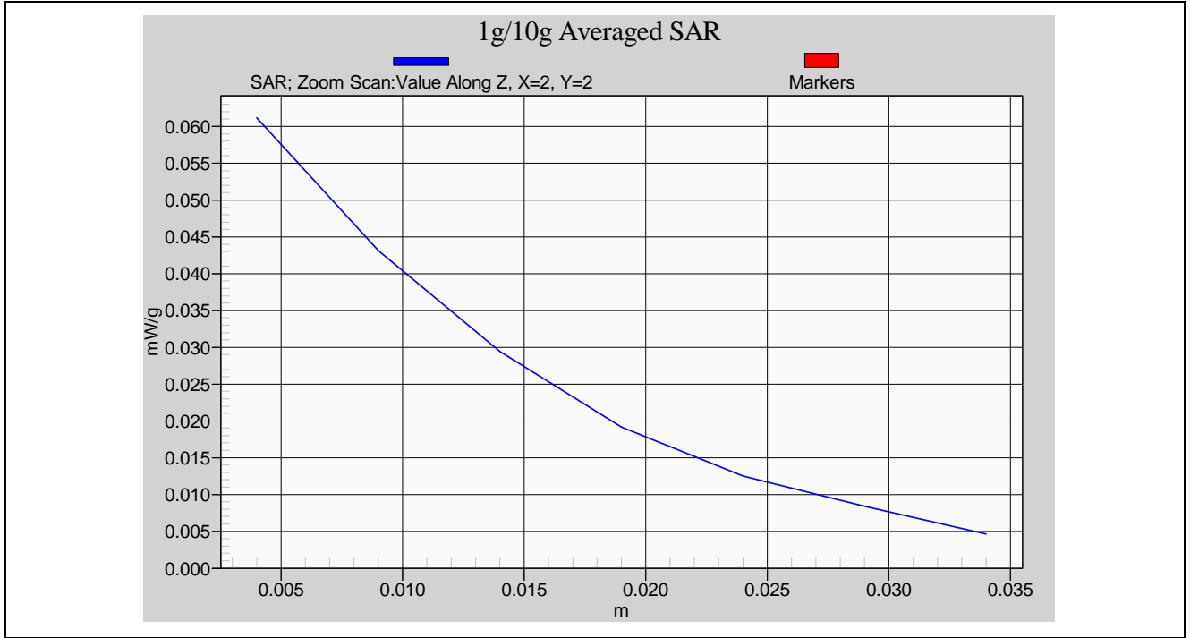
Head SAR Measurement _ Right Cheek CH0
