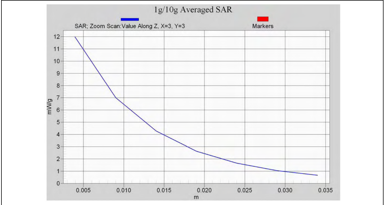
Body-Tissue-Simulating-Liquid 1950MHz (2008/07/30)
