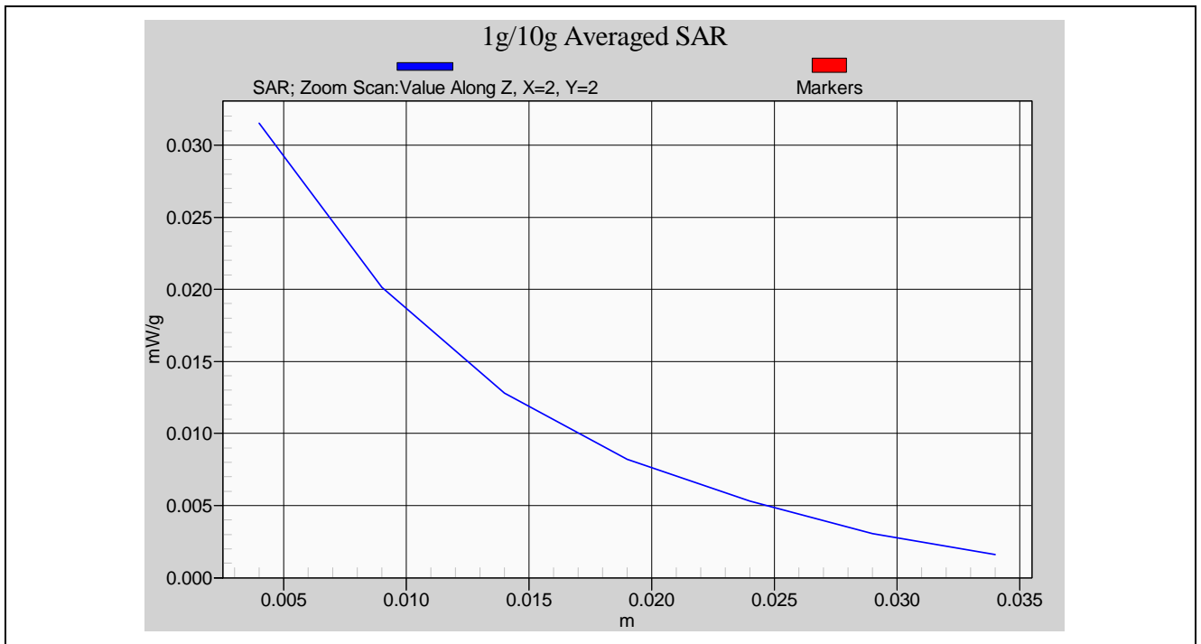
Body SAR Measurement _ Back to Phantom with Headset & Belt Clip NO.2_CH4
