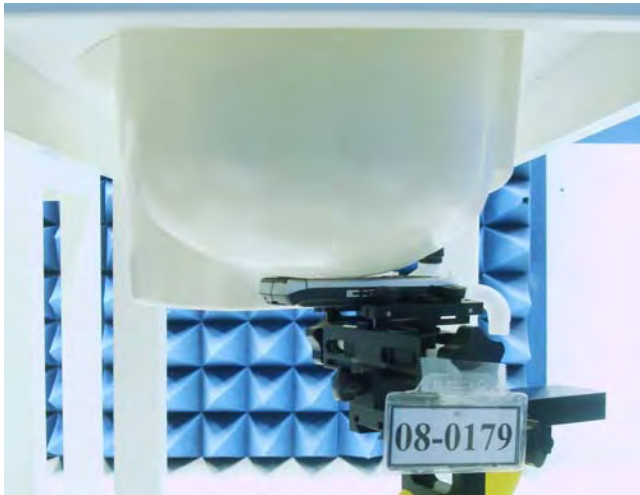
Figure 17. Right Head SAR Test Setup (Cheek)
