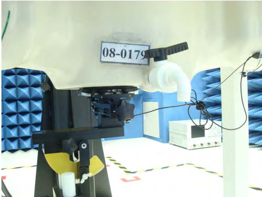
Figure 23. Body SAR Test Setup _ Back to Phantom 0mm separation
