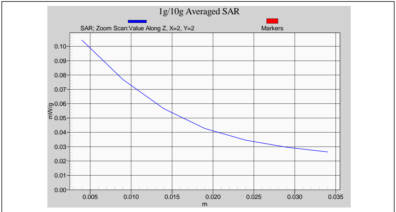
Body SAR Measurement _ Back to Phantom 0mm separation _ CH0
