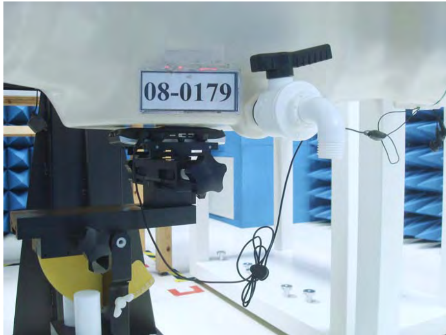
Figure 21. Body SAR Test Setup _ Back to Phantom with Headset & Belt Clip NO.1
