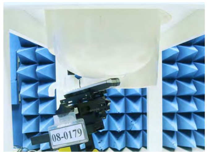
Figure 20. Left Head SAR Test Setup (Tilted)
