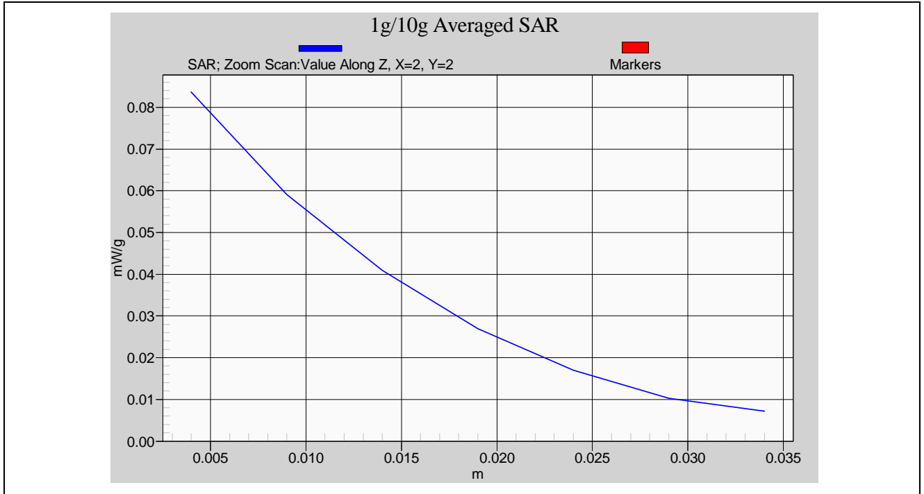
Body SAR Measurement _ Back to Phantom with Headset & Belt Clip NO.1_CH0
