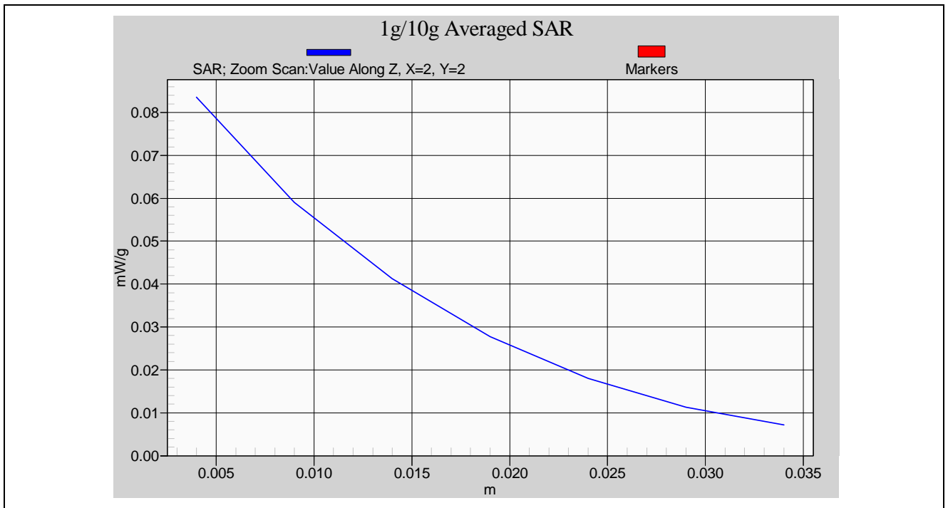
Body SAR Measurement _ Back to Phantom with Headset & Belt Clip NO.1_CH2
