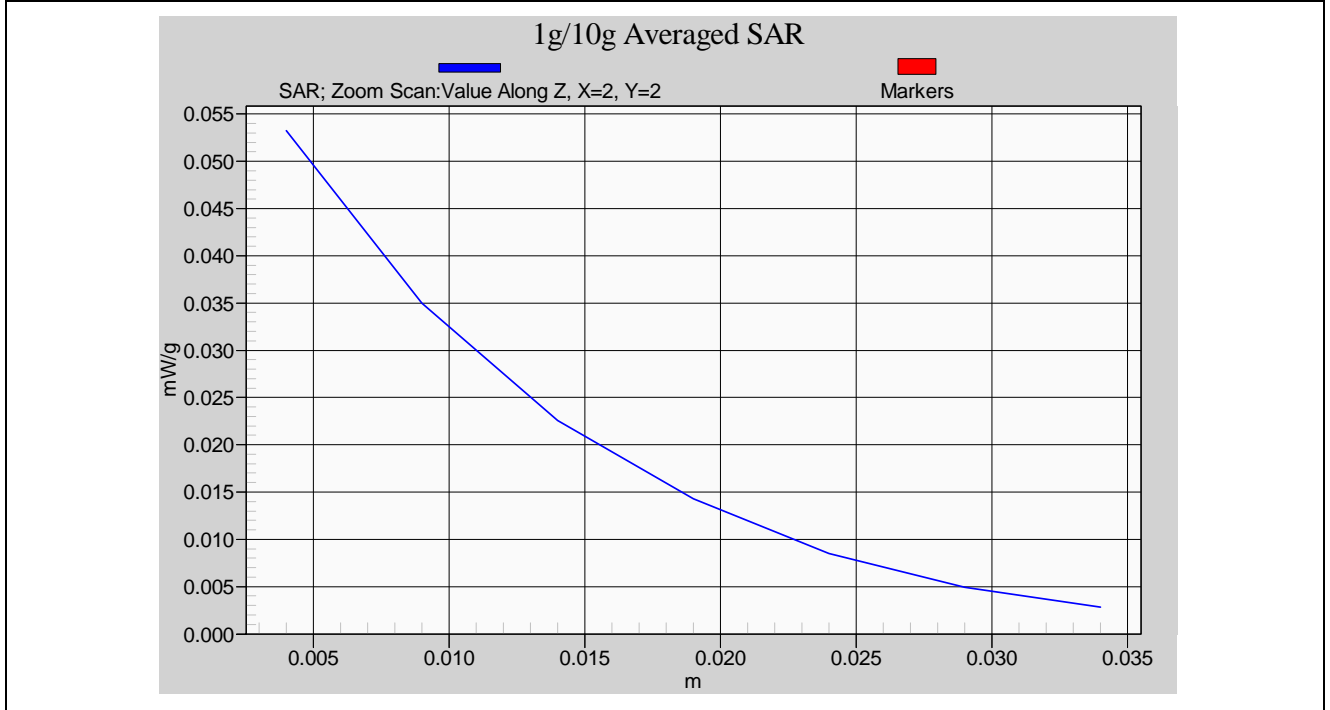
Body SAR Measurement _ Back to Phantom with Headset & Belt Clip NO.2_CH2
