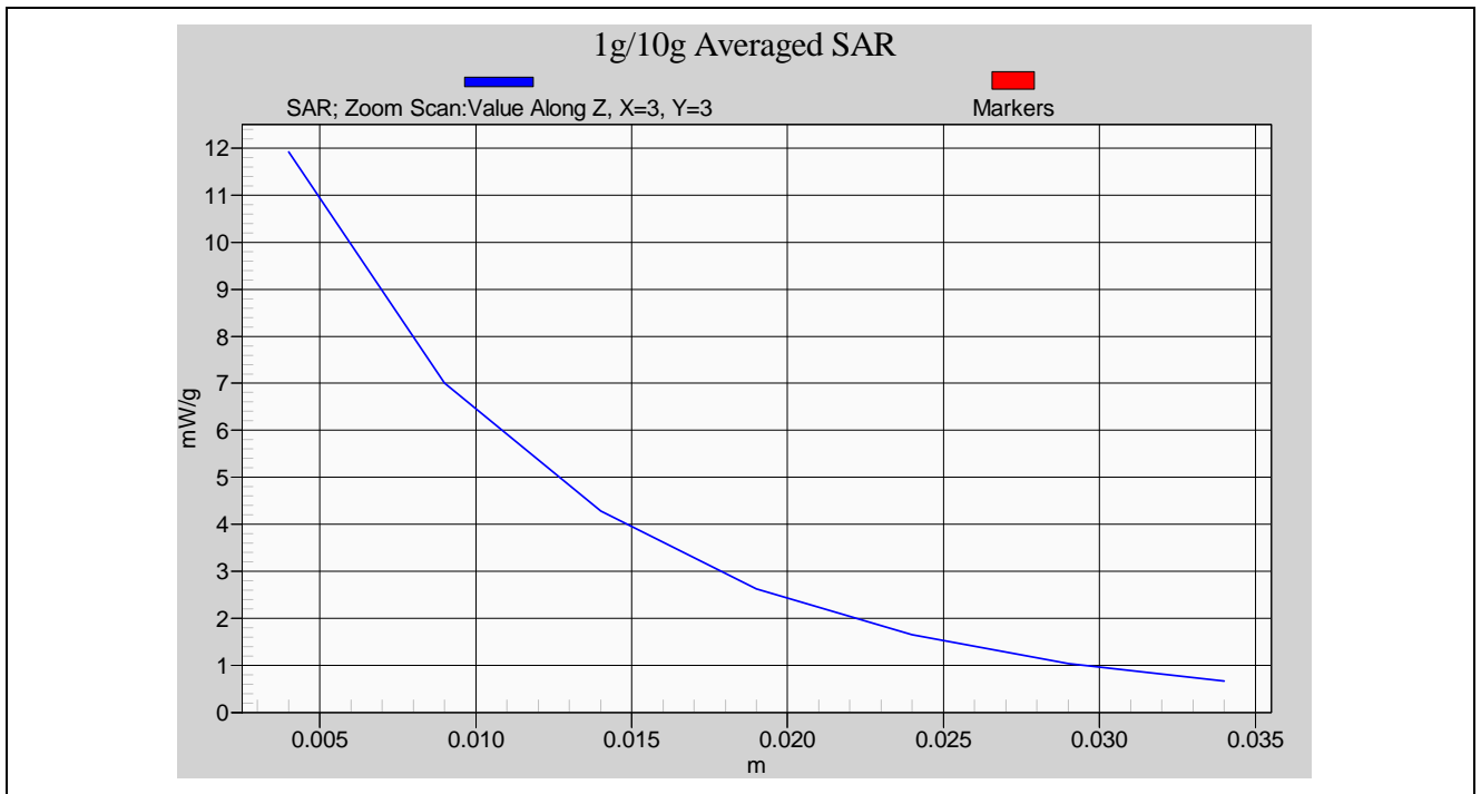
Body-Tissue-Simulating-Liquid 1950MHz (2008/07/07)
