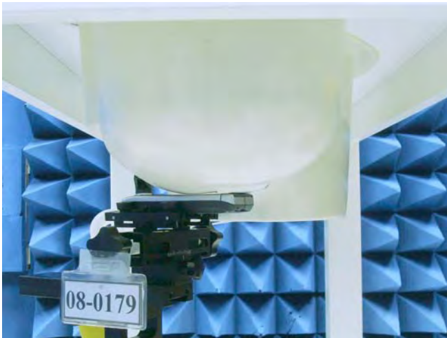
Figure 19. Left Head SAR Test Setup (Cheek)
