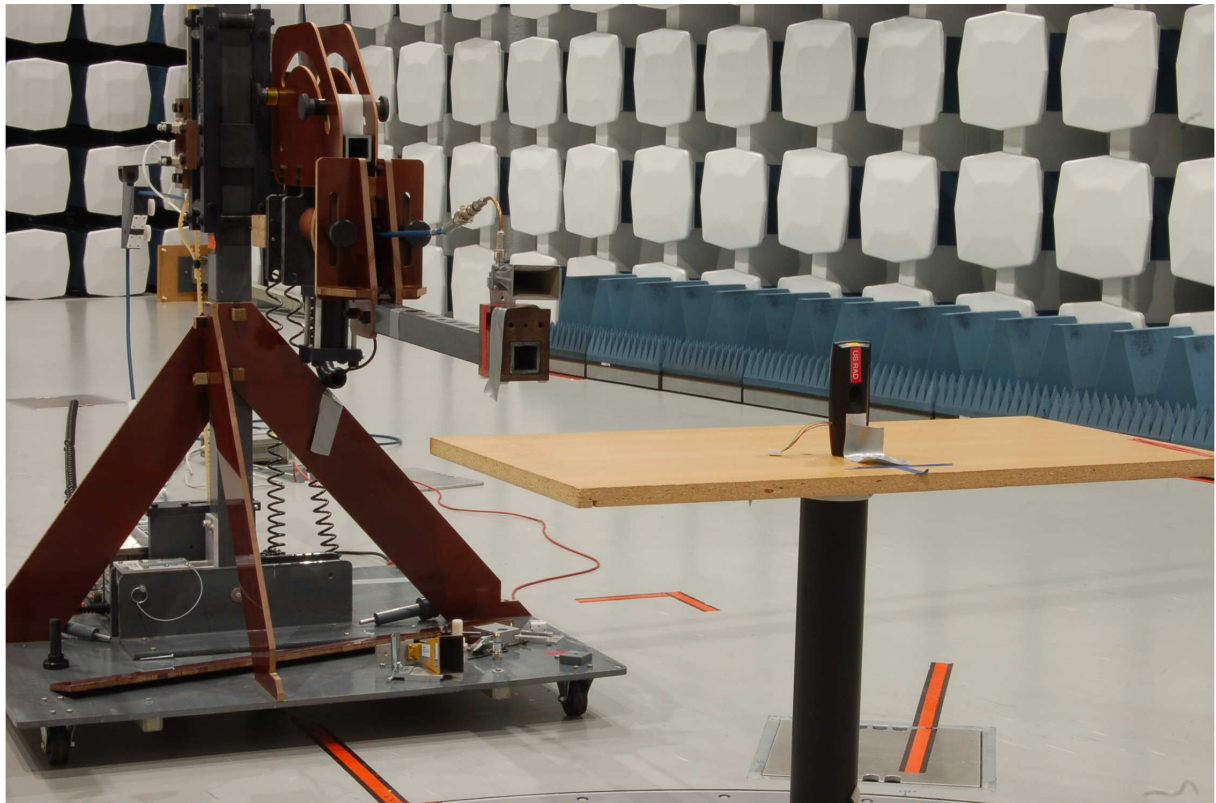
CT7141H-US - Radiated emissions 8.5 – 12 GHz
