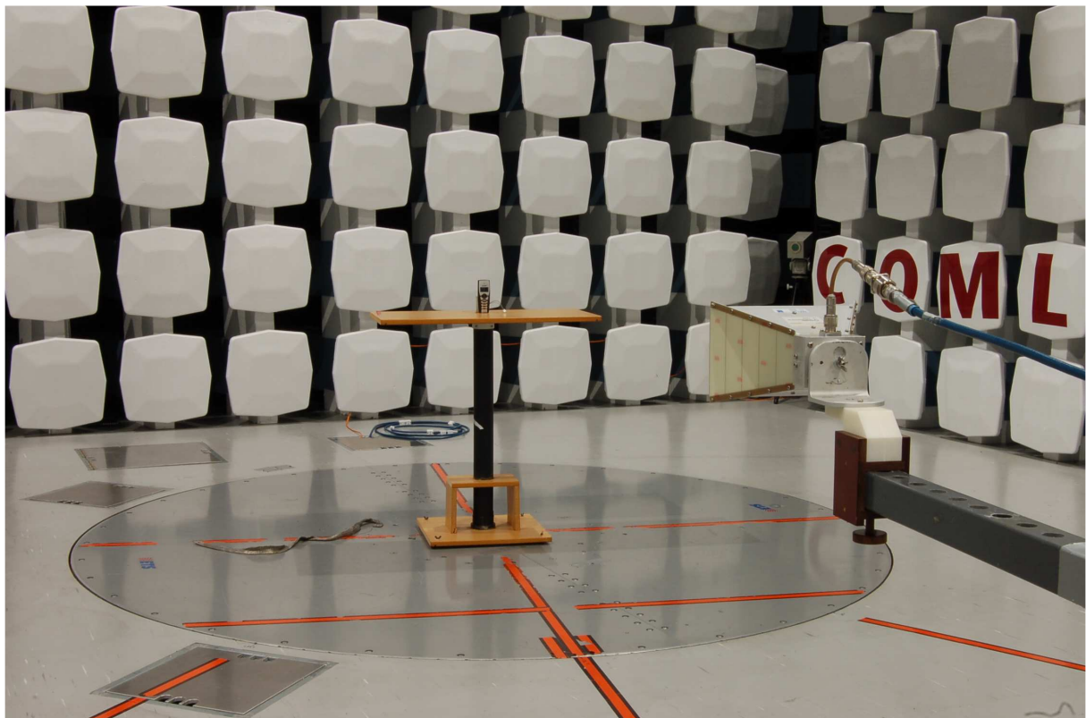
CT7141H-US - Radiated emissions 1 GHz - 8.5 GHz
