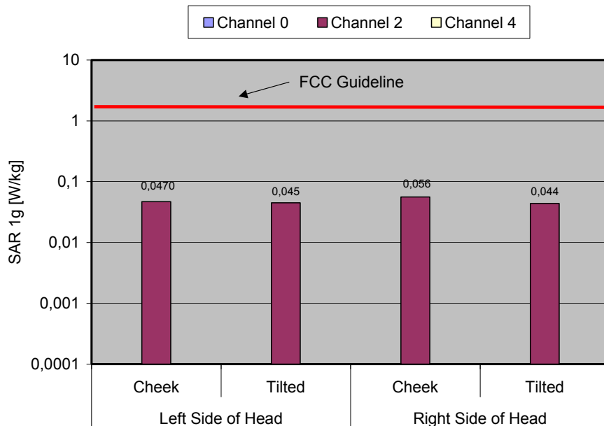
Fig. 8: The measured head phantom SAR values for the Webstar CT714H-US, with antenna 1 for the US DECT standard in comparison to the FCC exposure limit.
