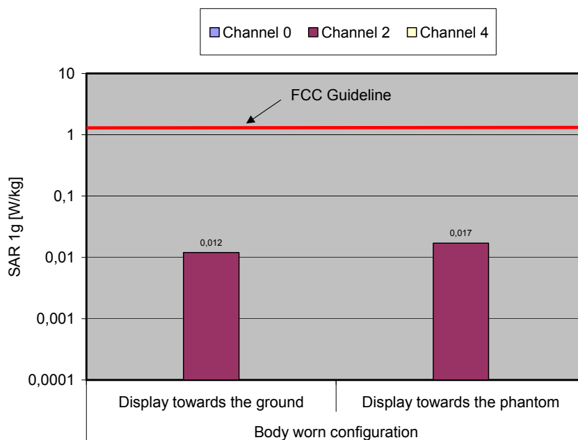
Fig. 9: The measured SAR values in body-worn configuration for the Webstar CT714H-US for the US DECT standard in comparison to the FCC exposure limit.
