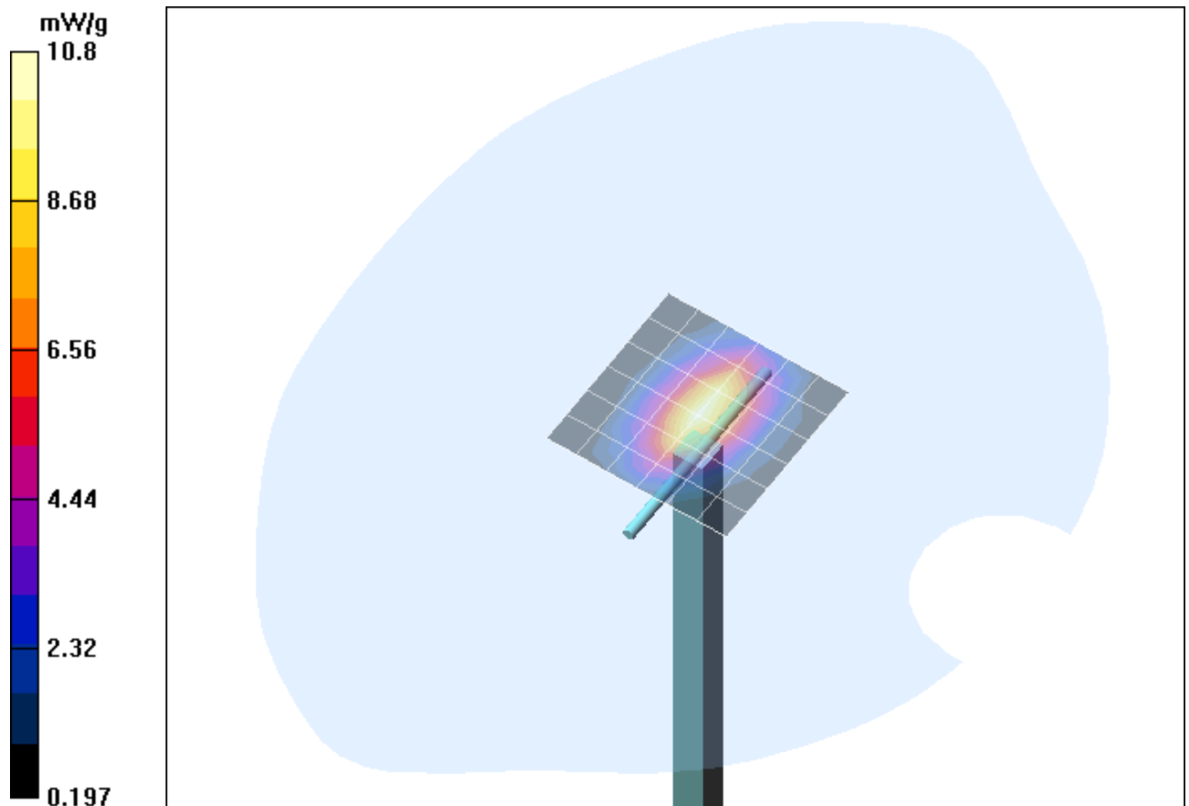
Fig. 10: Validation measurement 1900 MHz Head (May 10, 2006), coarse grid. Ambient Temperature: 21.8° C, Liquid Temperature: 20.7° C.
