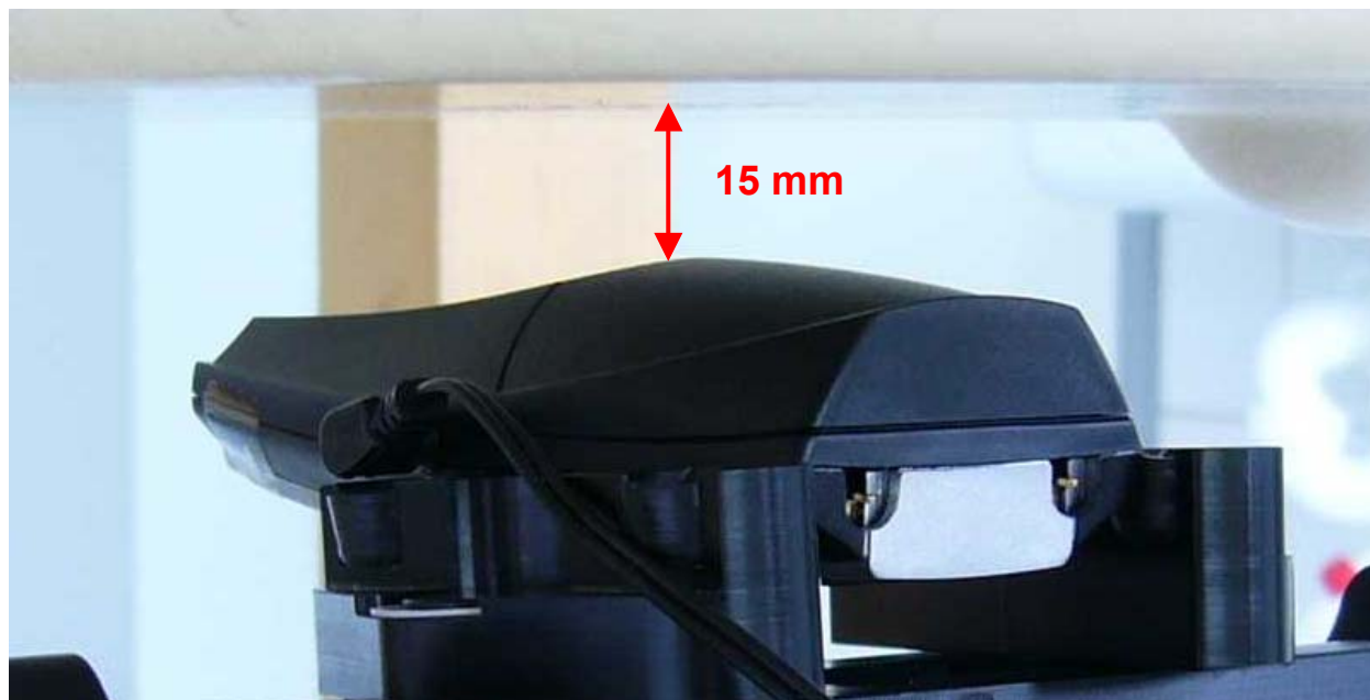
Fig. 20: Body worn configuration, with headset, display towards the ground.
