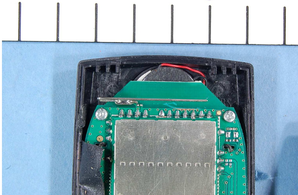
CT7141H-US, Antenna
