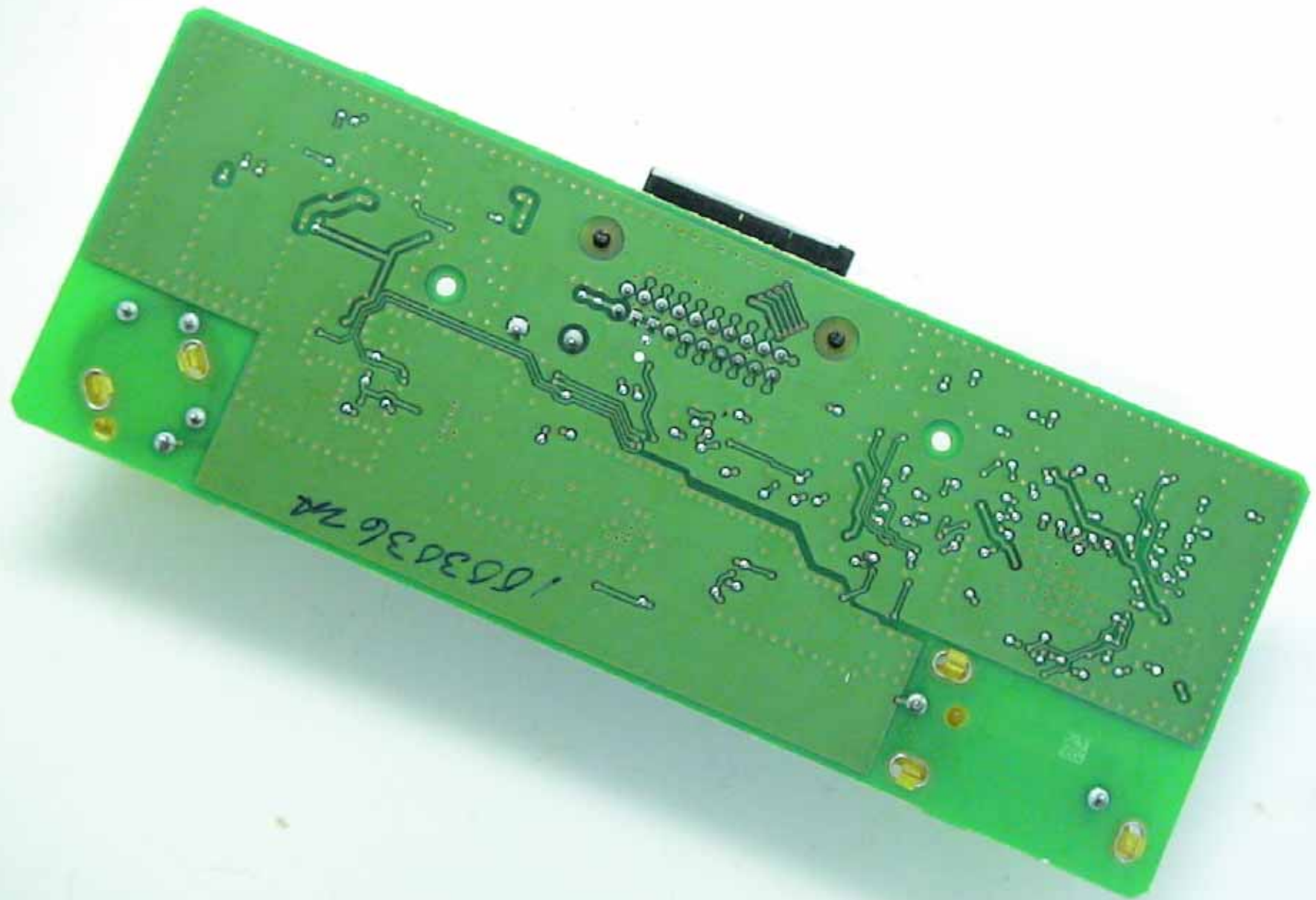
PCB (bottom)
