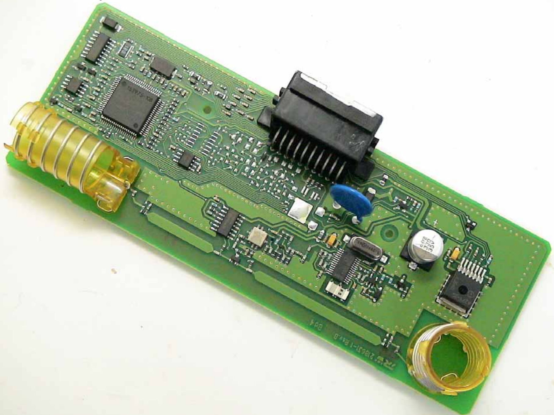
PCB (top)
