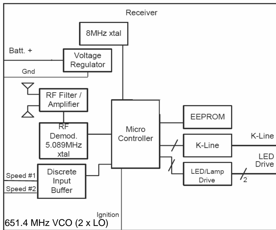
Figure 3. TPM Lowline Receiver Block Diagram
