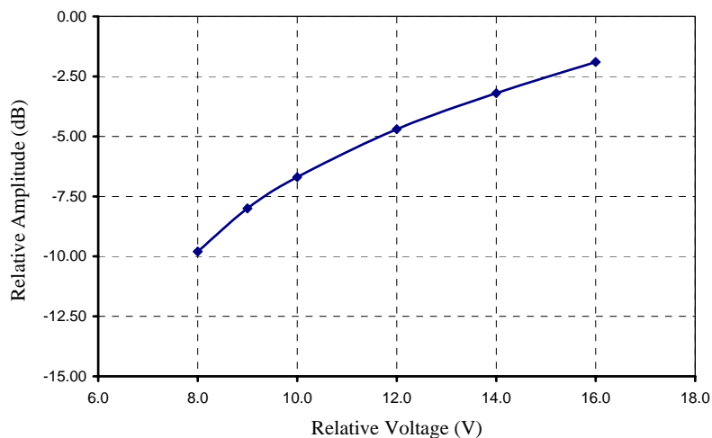
Figure 6.4. Relative emission at 135 kHz vs. supply voltage.
