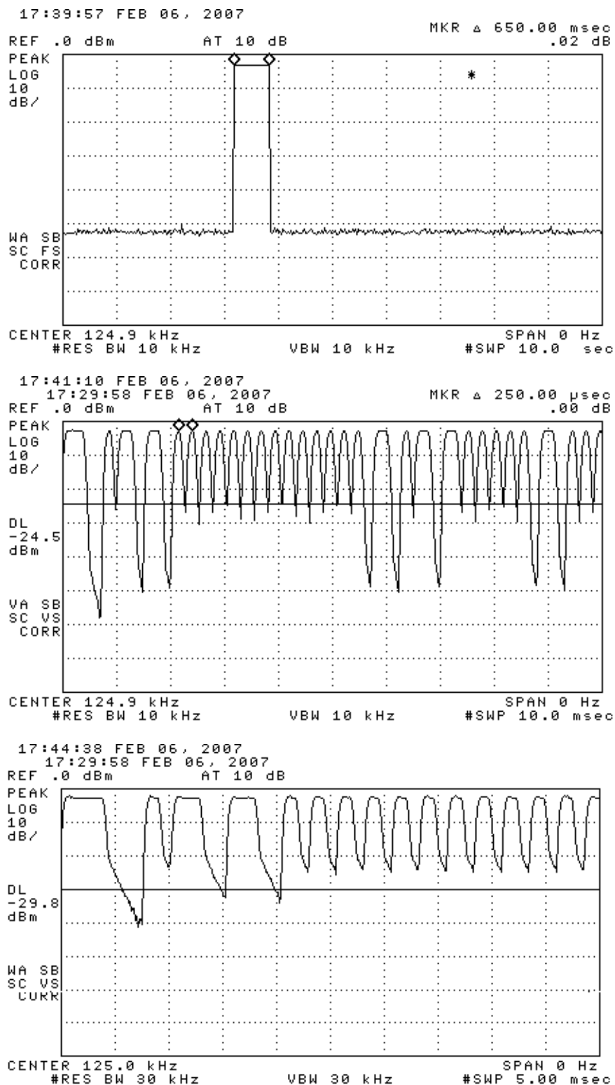
Figure 6.1. Transmission modulation characteristics. (top) On time, (middle) Manchester encoding, (bottom) leading pulse
