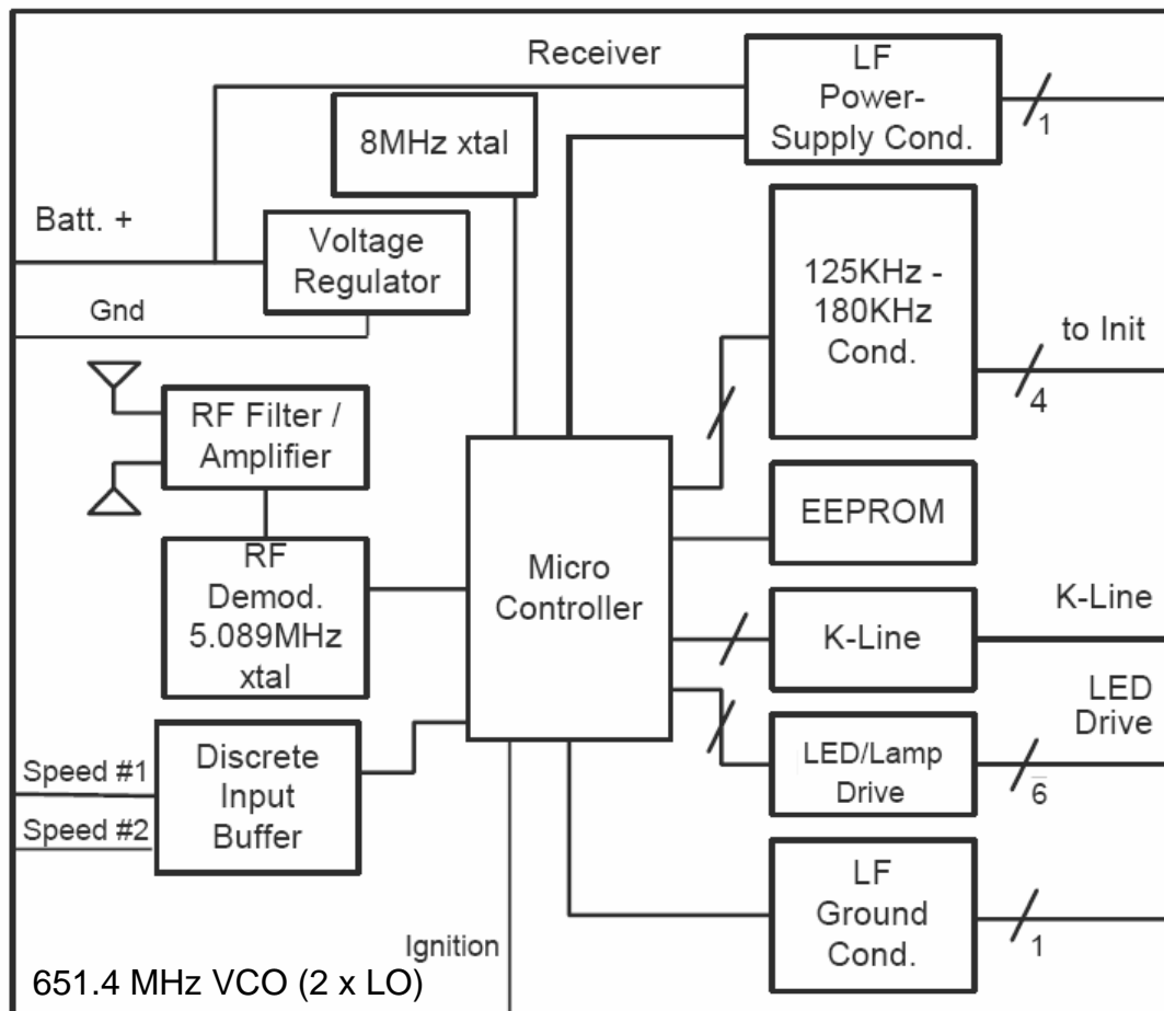
Figure3. TPM Receiver Block Diagram
