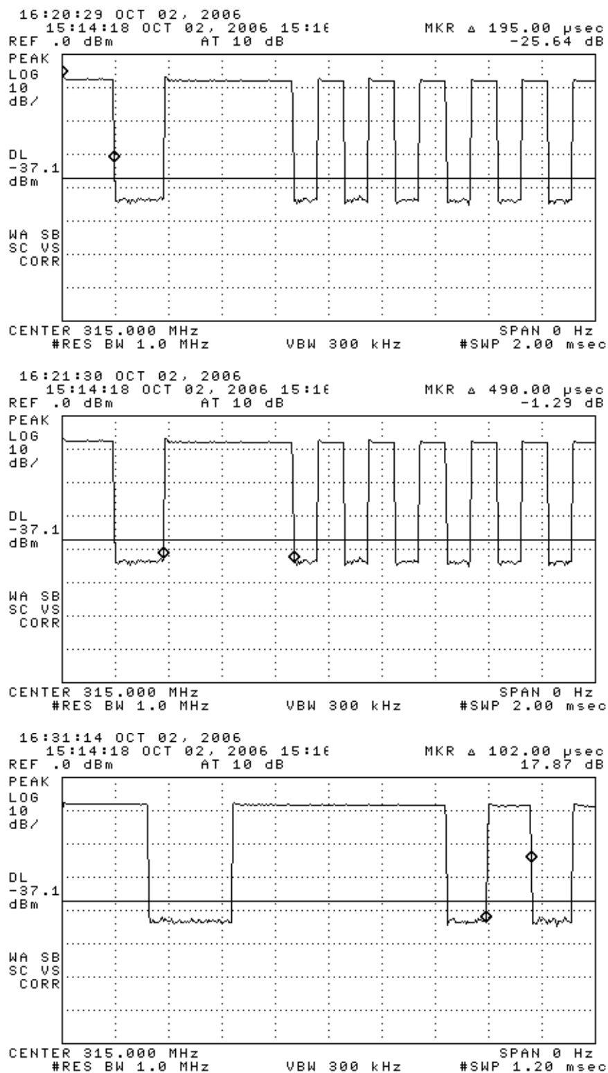
Figure 6.1(b). Transmissions modulation characteristics: (top) wake pulse 1, (center) wake pulse 2, (bottom) Manchester pulse.
