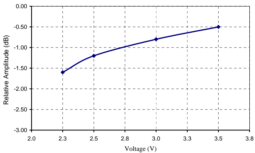
Figure 6.4. Relative emission at 315.0 MHz vs. supply voltage (cw emission).
