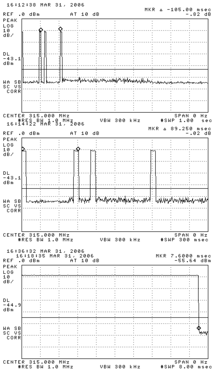
Figure 6.1. Transmissions modulation characteristics: (top) complete transmission, (bottom) expanded FSK word.
