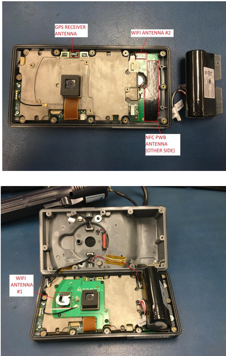
Figure 1 Antenna Locations Internal to Device
