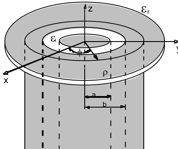
Figure 8.2.1. An open-ended coaxial probe with inner and outer radii a and b , respectively
