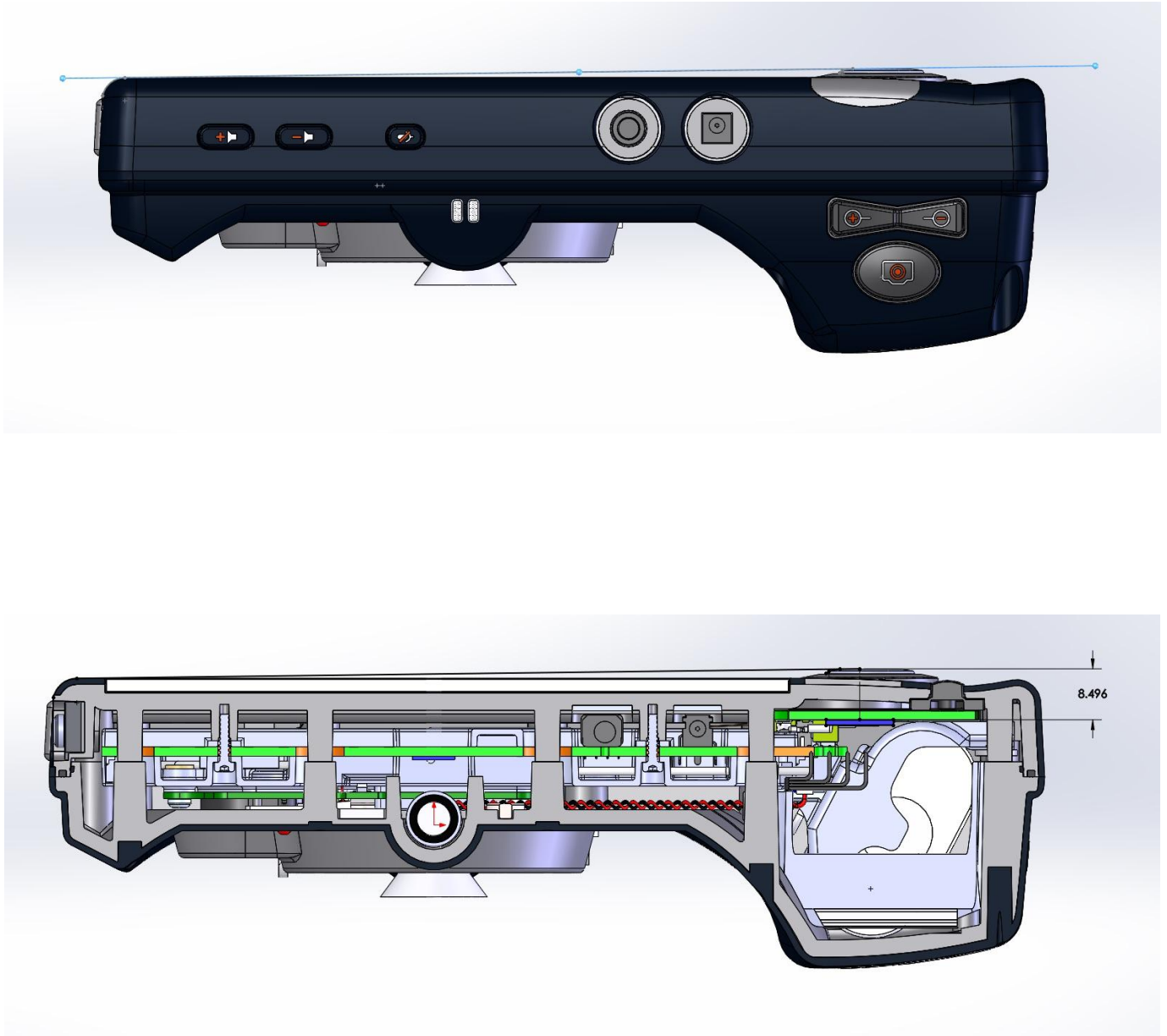
Figure 2 Top Antenna 2 - Separation Distance to back touch plane
