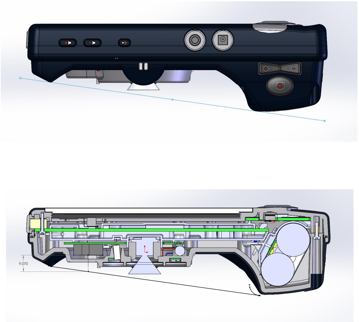
Figure 3 Front Antenna 1 - Separation distance to front touch plane
