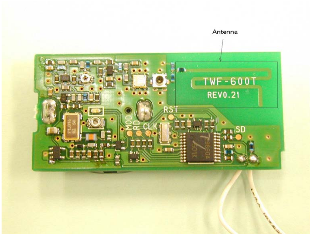
Component side with Antenna specified
