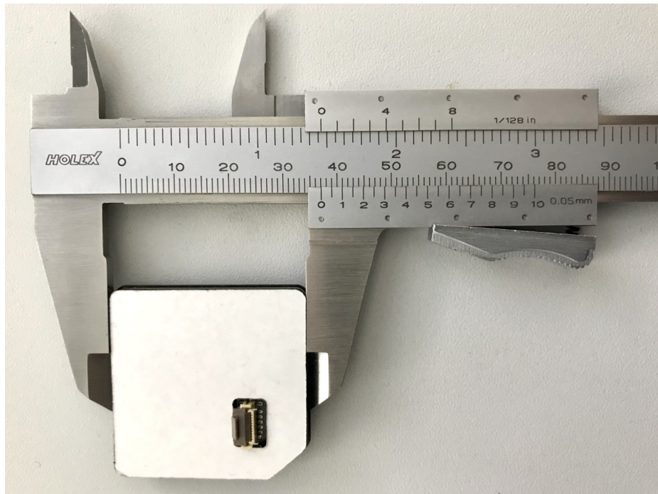
Board outline according PCB: 36.2 mm * 37.1 mm
