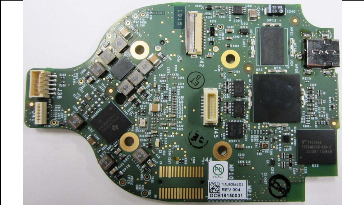
Figure 11 TIX560 Series Main Processing Circuit Board (Bottom Side, Identical For All Models)
