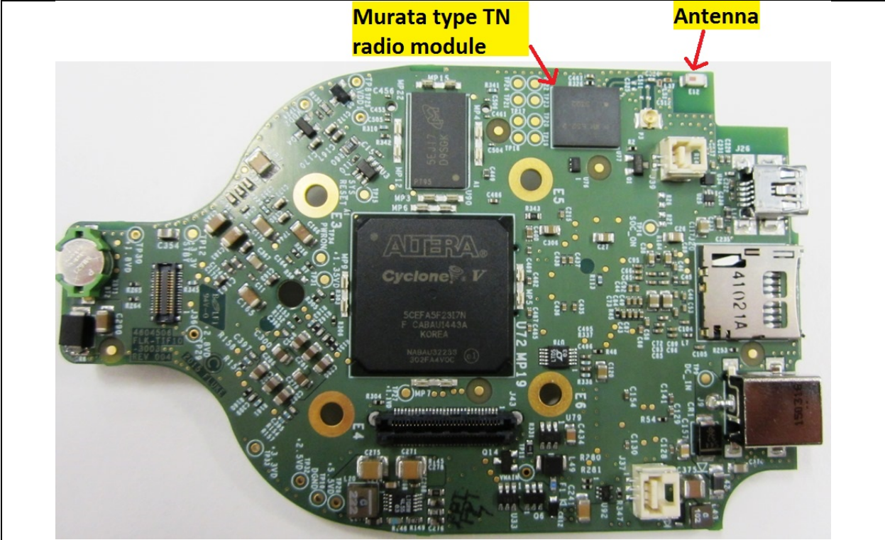
Figure 10 Main Processing Circuit Board (Top Side, Identical For All Models)
