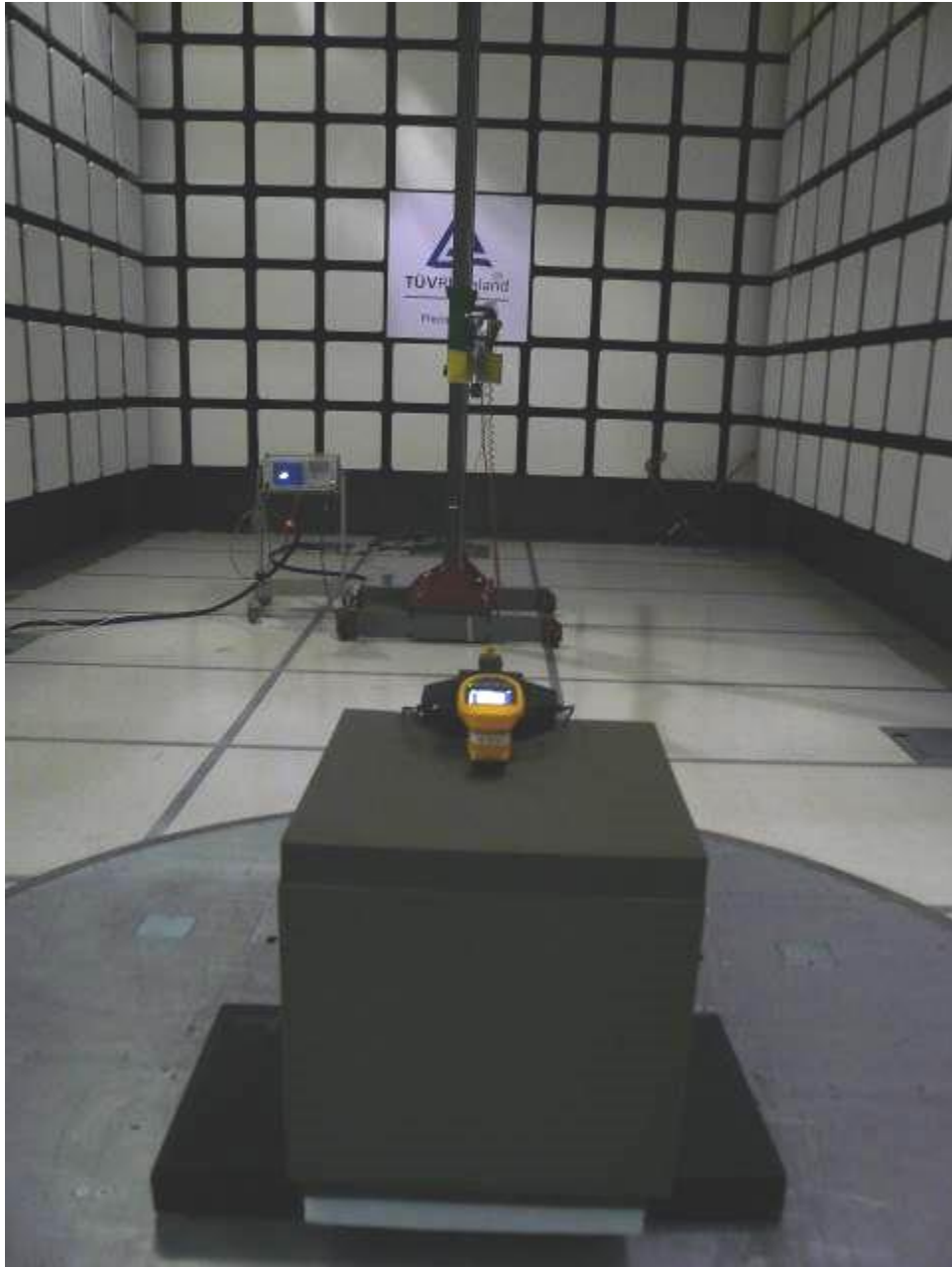
Radiated Emissions 1 to 18GHz
