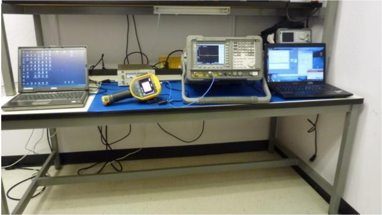
Test setup Conducted TX measurements
