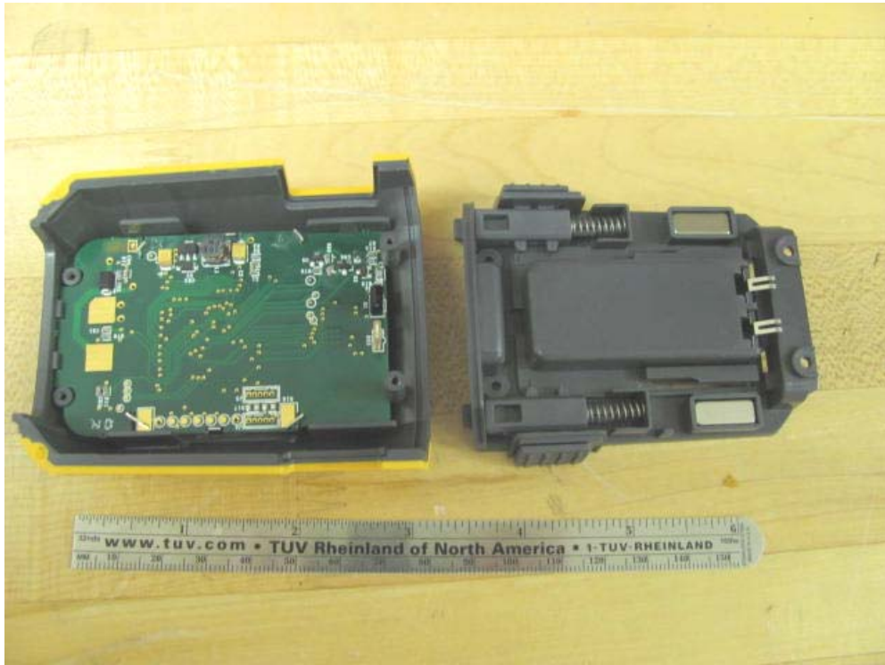
Figure 1: View with battery compartment off.
