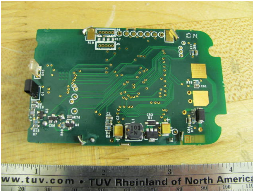
Figure 3: Top View of PCB.
