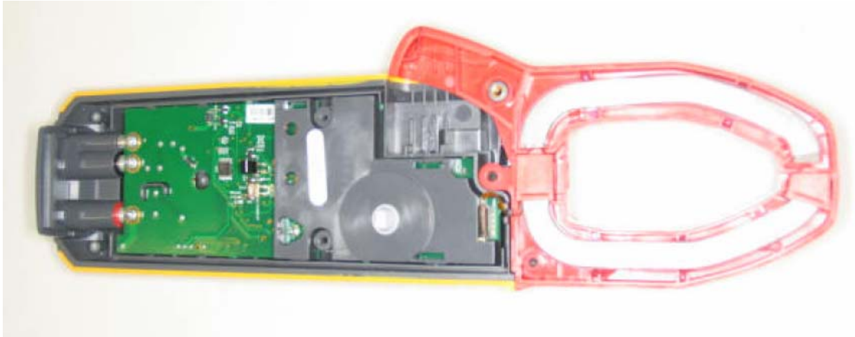
Figure 1: View with back cover off.
