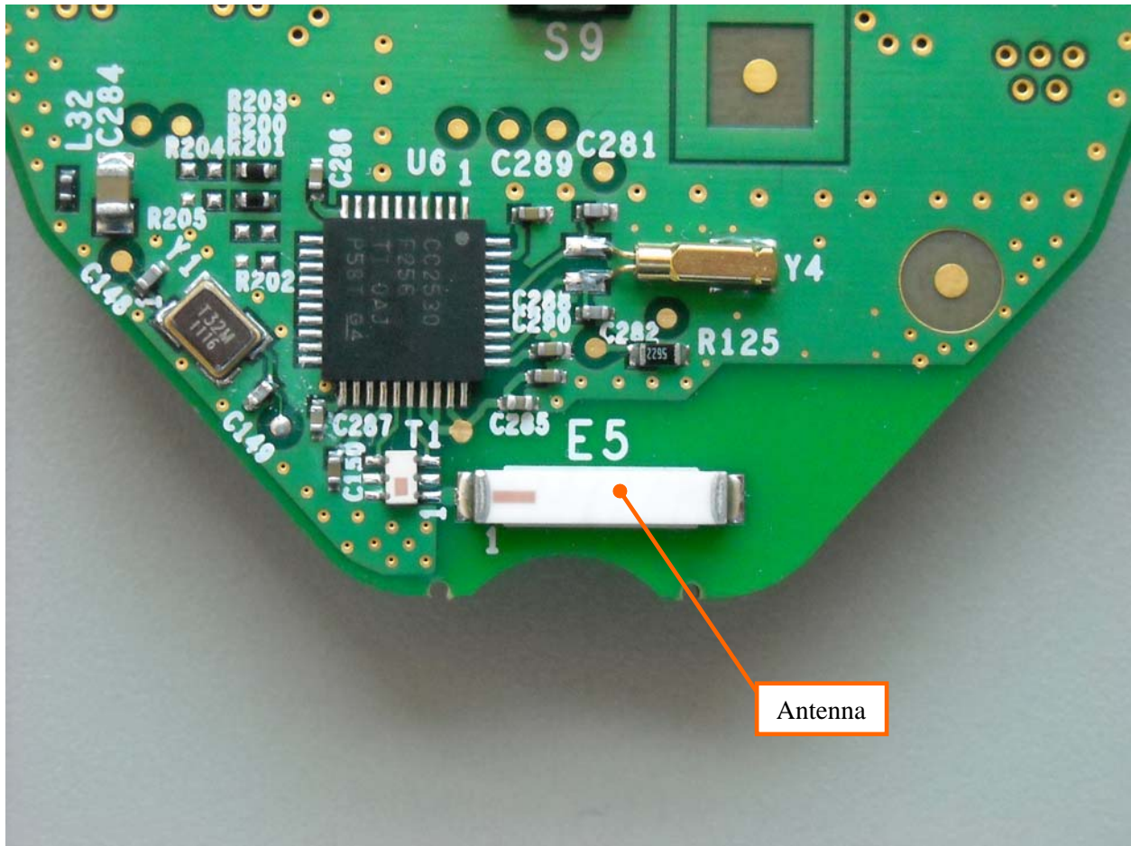
Figure 4: Close up View of the transmitter section.
