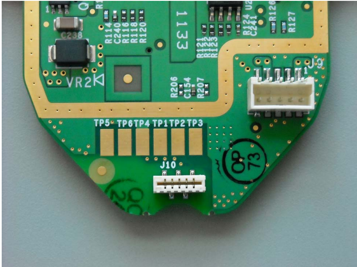
Figure 3: Top close up bottom view of transmitter section of main board.
