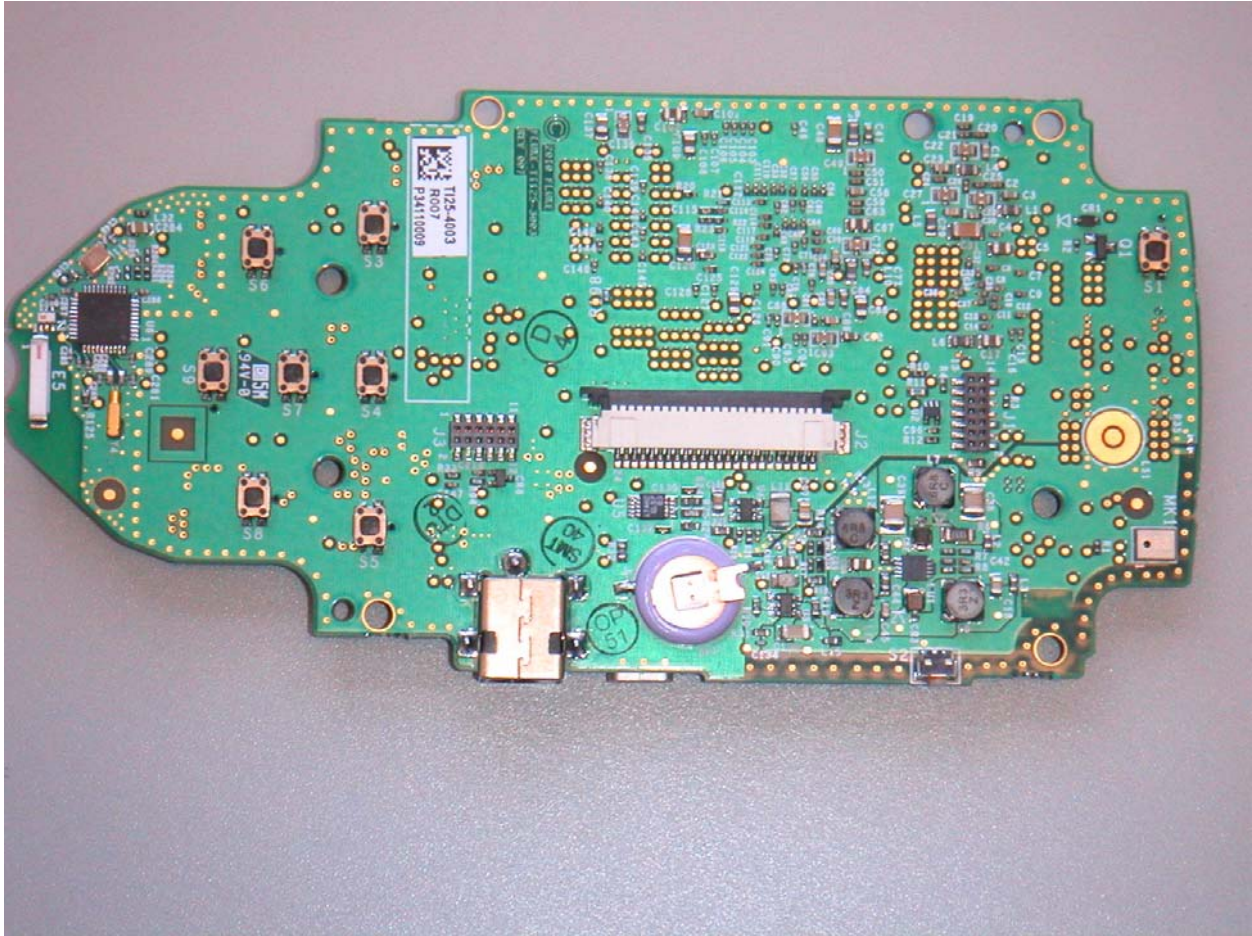
Figure 1: View with main board with transmitter.
