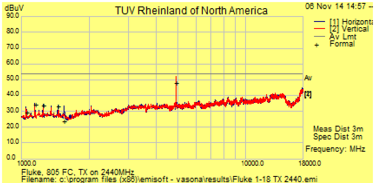
Above 1 GHz Radiated Emission Plot for Transmit Mode at 2440 MHz, 1Mbit/s
