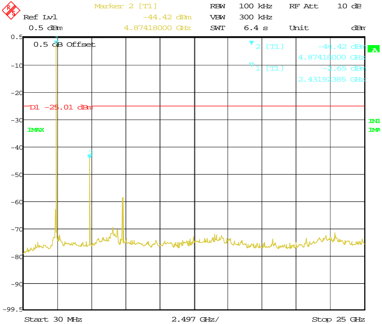
Figure 18: Out of Band Emission Requirements at 2440 MHz
