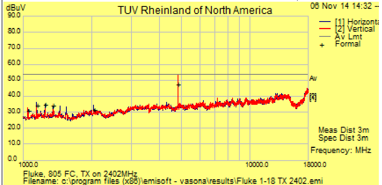
Above 1 GHz Radiated Emission Plot for Transmit Mode at 2402 MHz, 1Mbit/s
