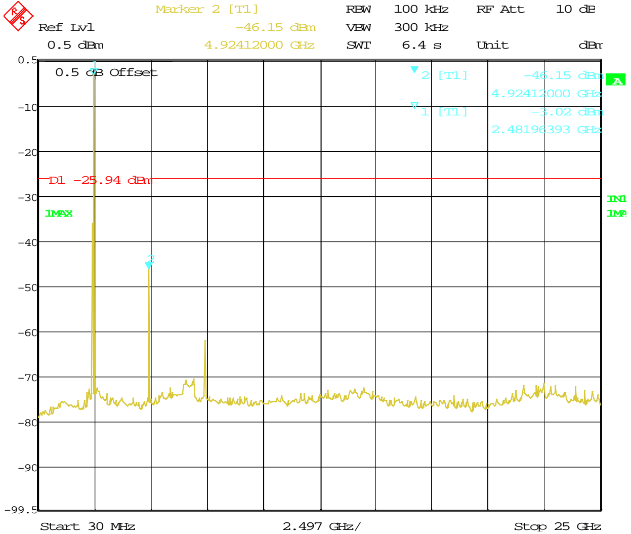
Figure 19: Out of Band Emission Requirements at 2480 MHz
