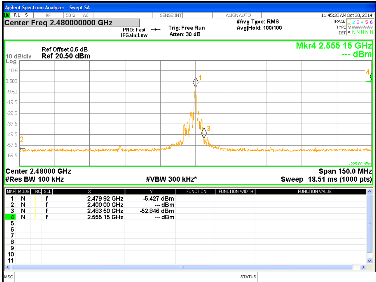
Figure 16: Band Edge Requirements at 2480 MHz
