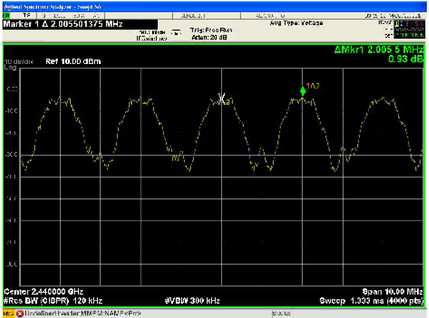
Figure 12: Channel Separation at 2440MHz
