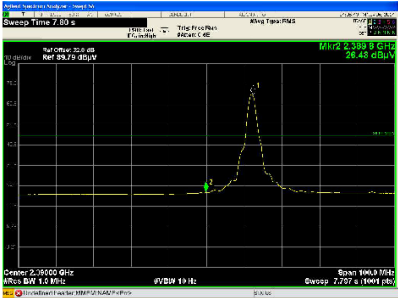
Figure 23: Radiated Emission at the Edge for Channel 2402 MHz at 1Mbps – Horizontal (avg)
