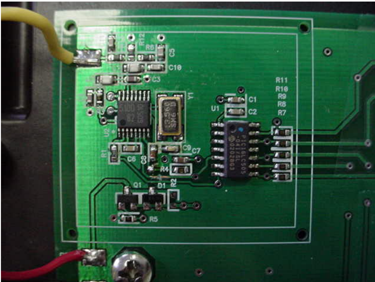
Photo Two – Internal Close-Up of RF Section
