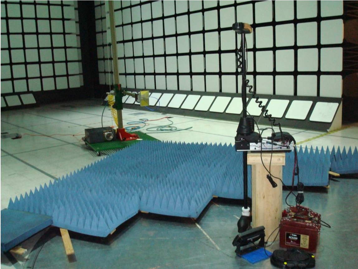
Figure 3 - Radiated Emissions Test Setup
