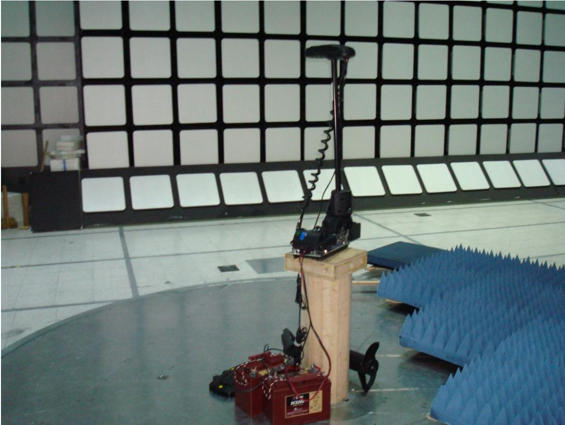
Figure 4 - Radiated Emissions Test Setup
