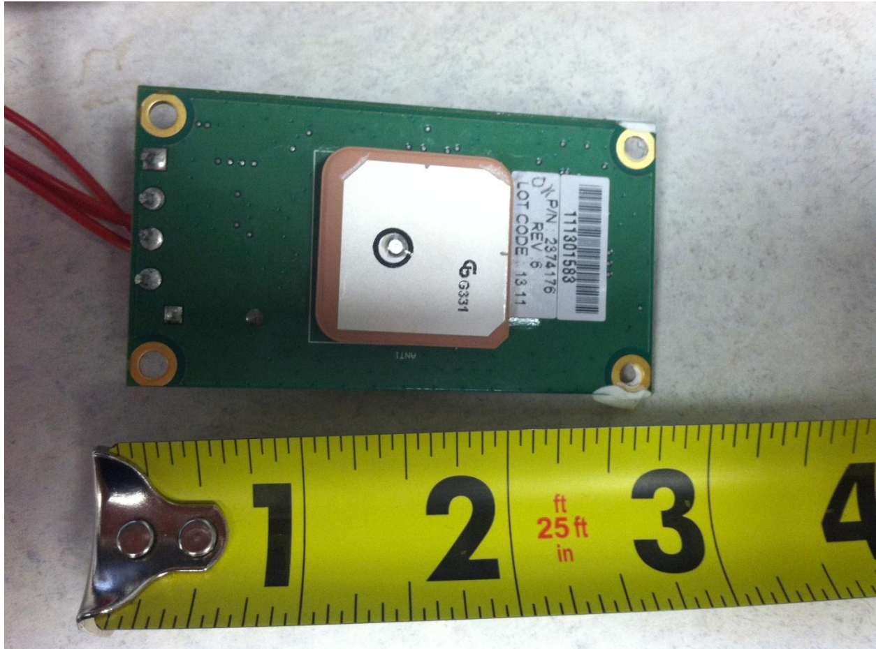
Figure 19 - iPilot Standard Compass Board, bottom
