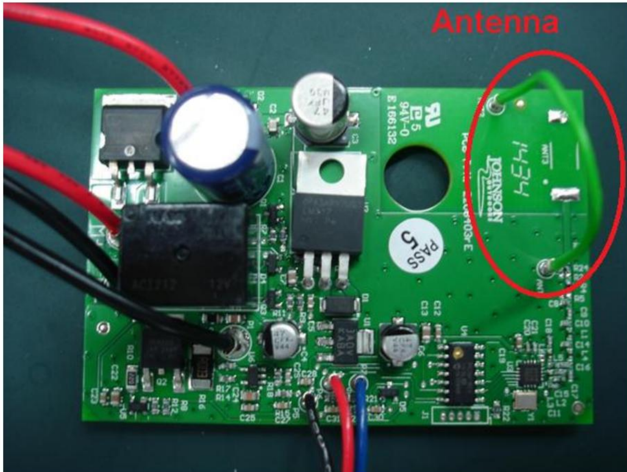
Figure 7 – Trim Board, Top
