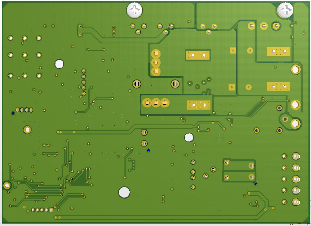
Figure 11 - Main Board, Back
