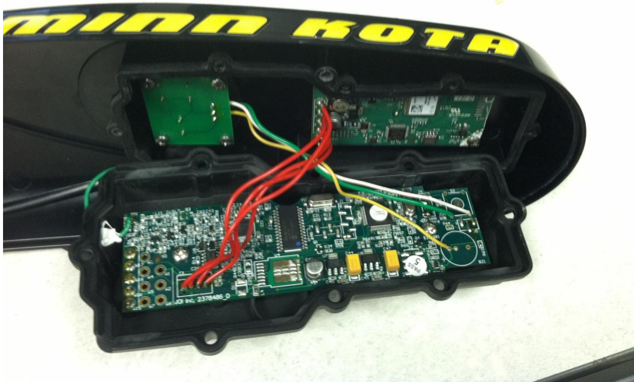
Figure 15 - iPilot Standard Head Underside opened
