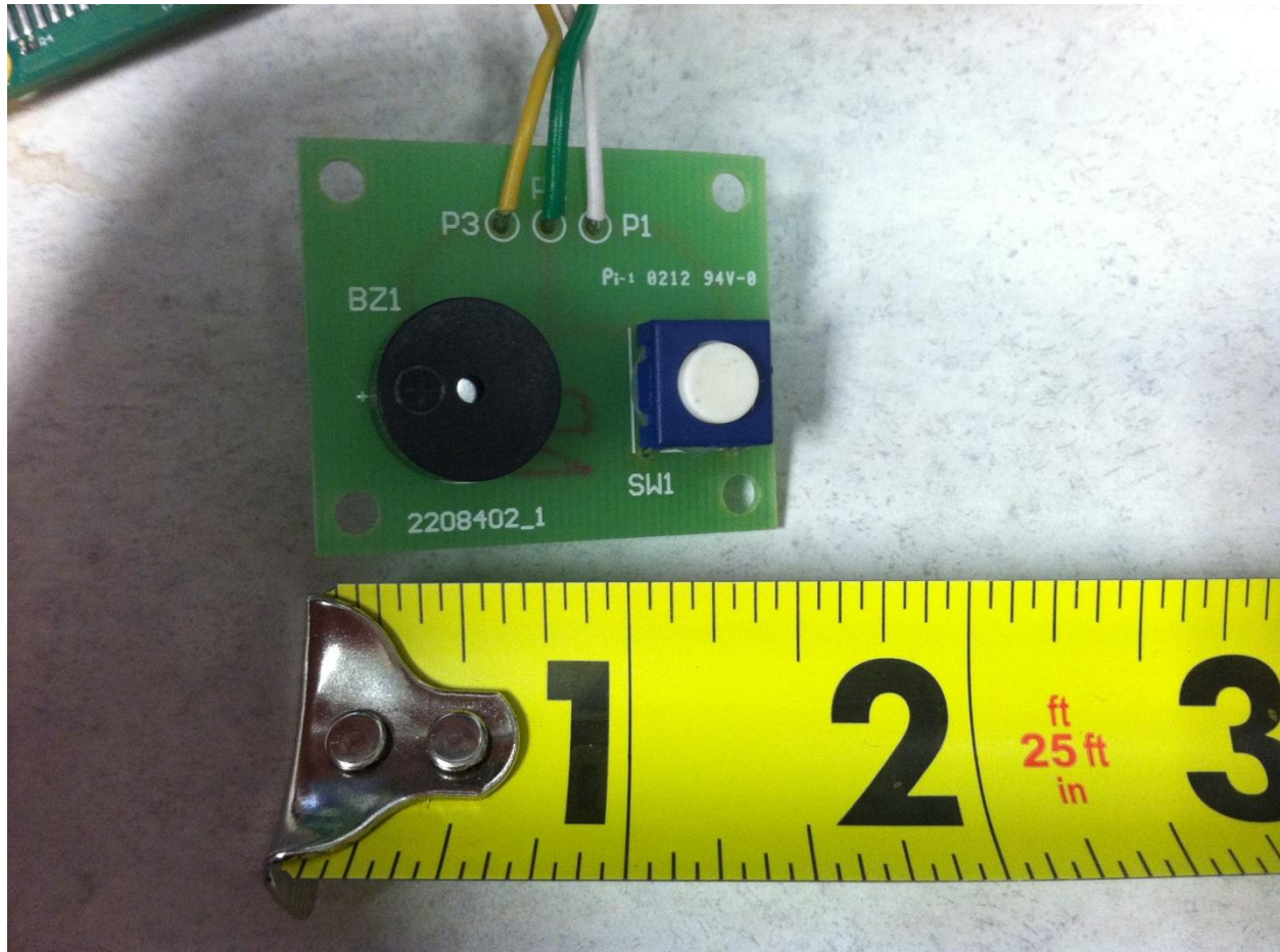
Figure 21 - iPilot Standard, push button and beeper board, top
