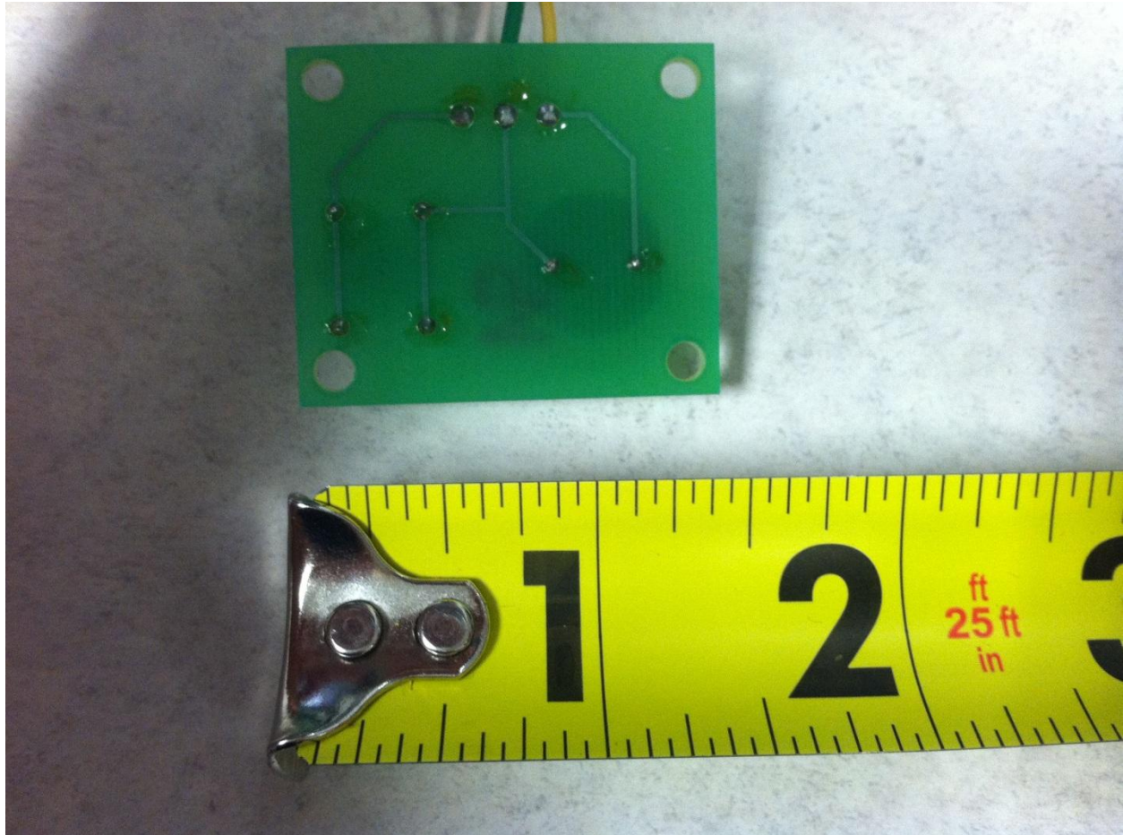
Figure 22 - iPilot Standard, push button and beeper board, top
