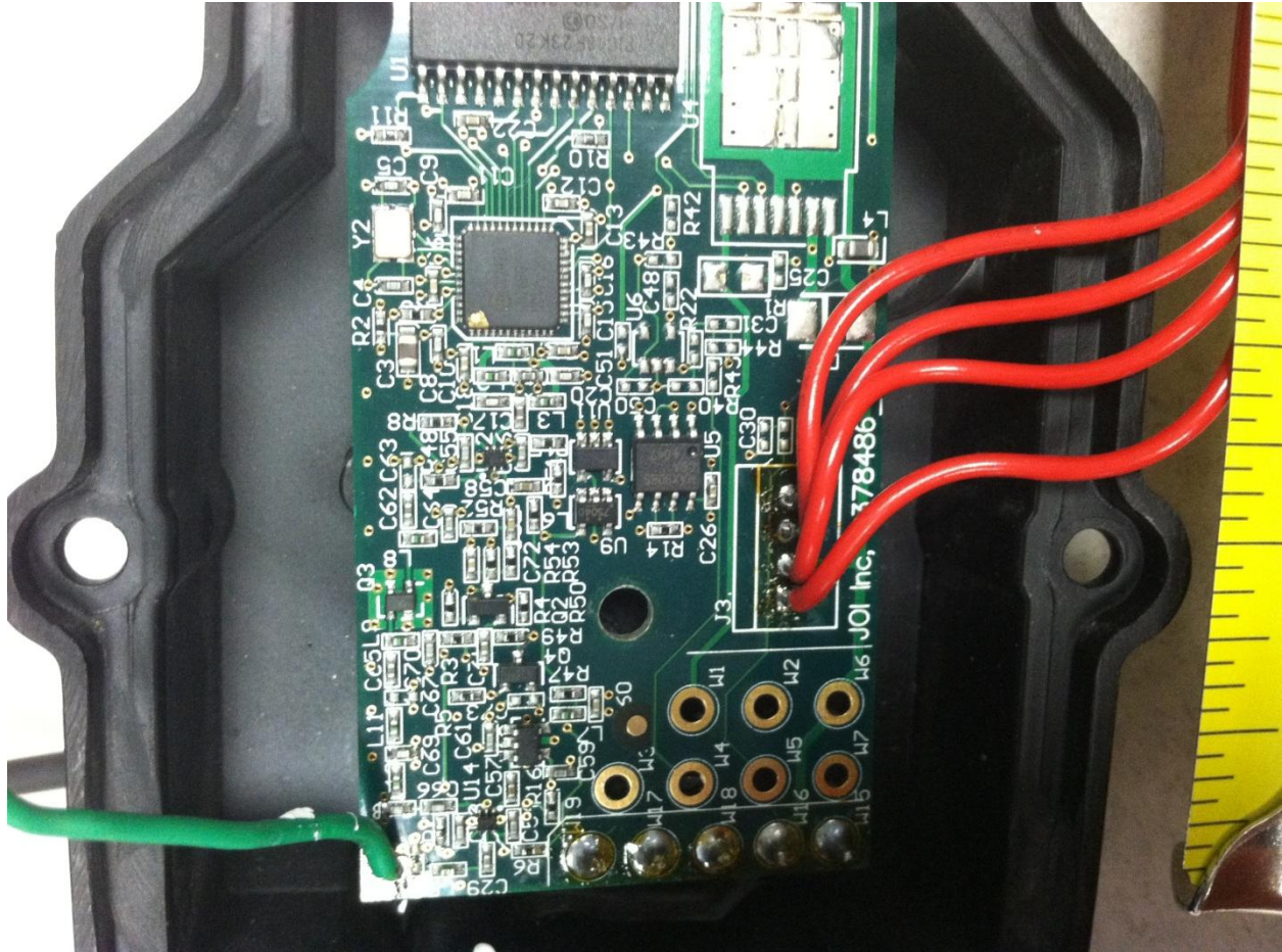
Figure 17 - iPilot Standard circuit board detail
