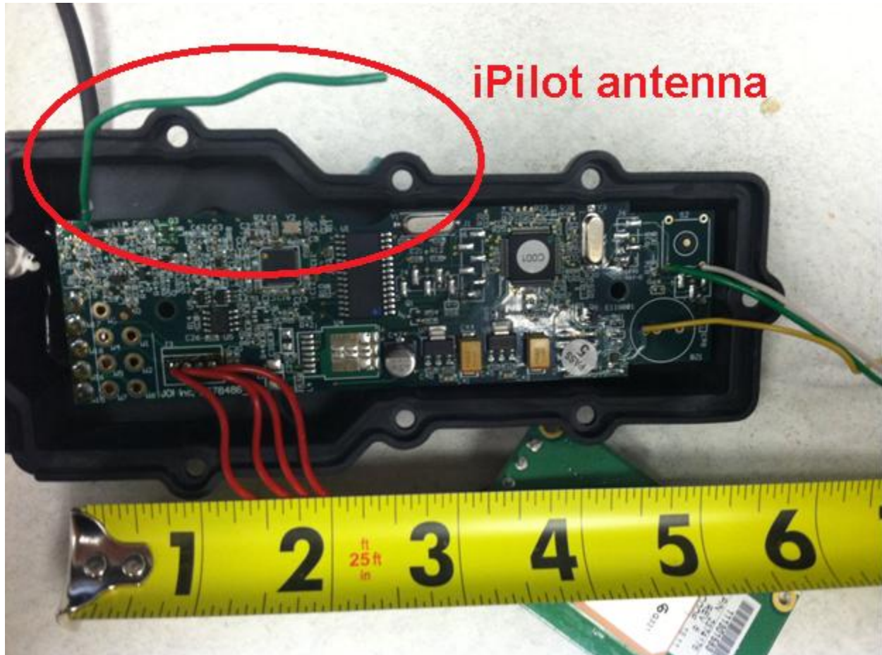
Figure 16 - iPilot Standard circuit board
