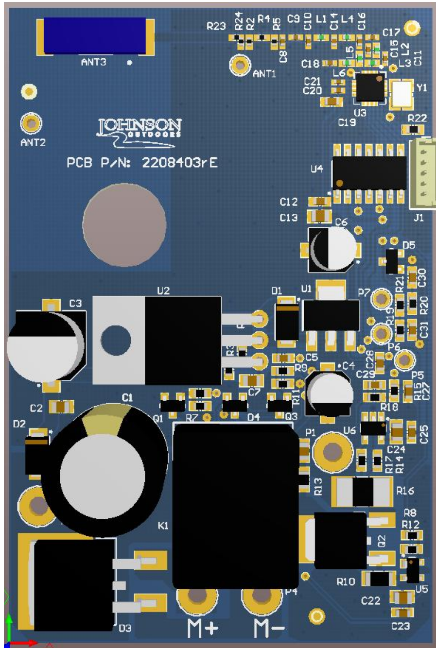
Figure 3 - Trim Board, Front
