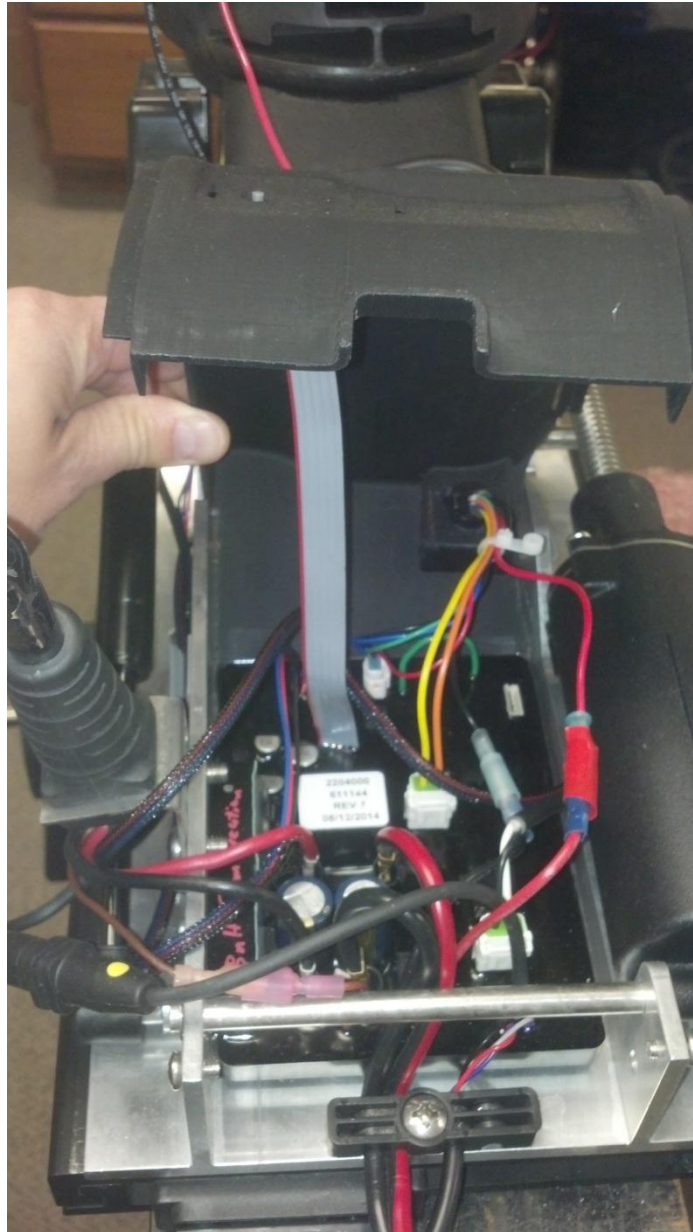
Figure 2 - Main board in assembly
