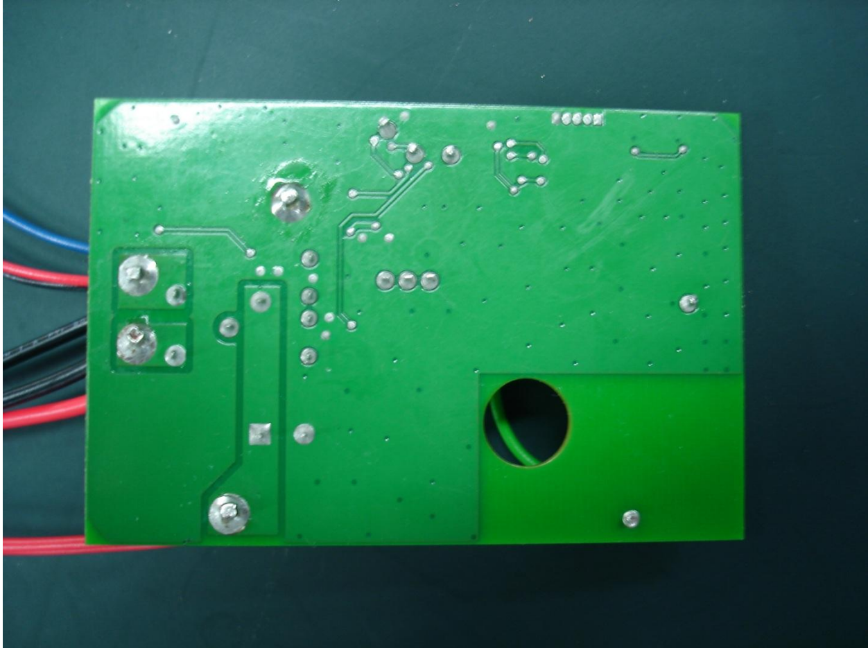
Figure 6 – Trim Board, Bottom
