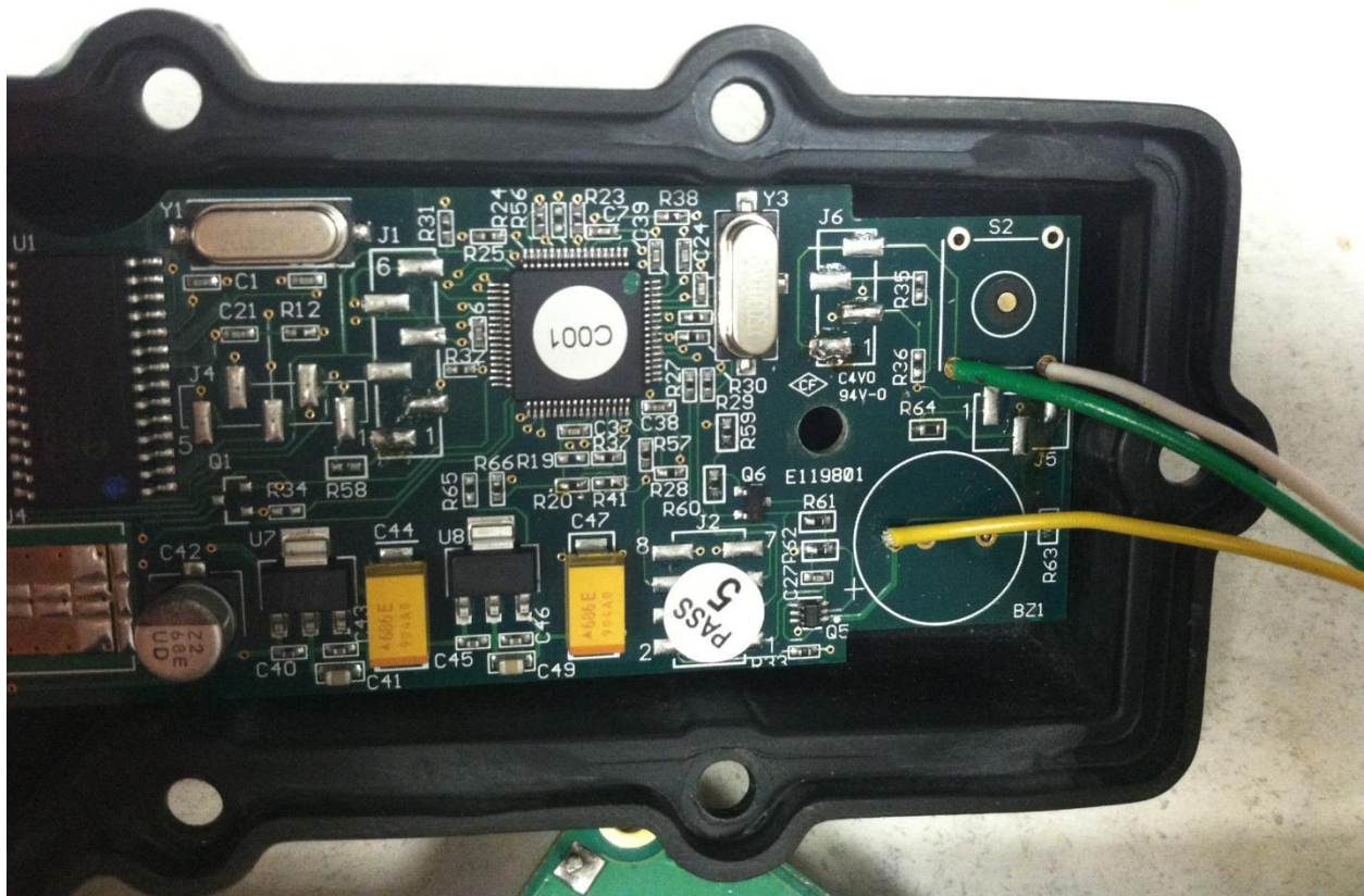
Figure 18 - iPilot standard circuit board detail
