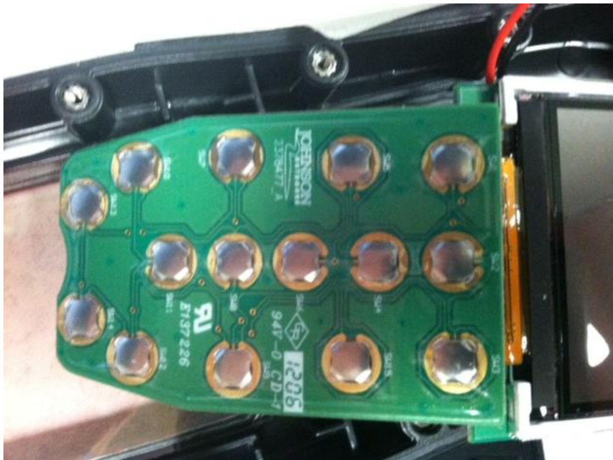
Figure 3 - Internal Photos, Keypad
