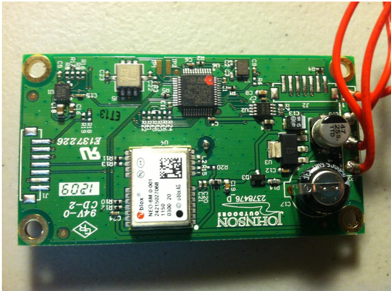
Figure 3 - Compass/combination board
