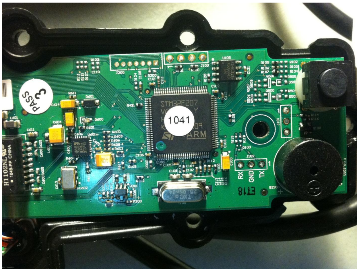
Figure 7 - RF Board detail
