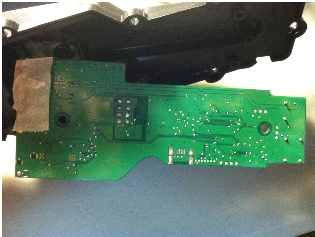
Figure 8 - RF Board, bottom
