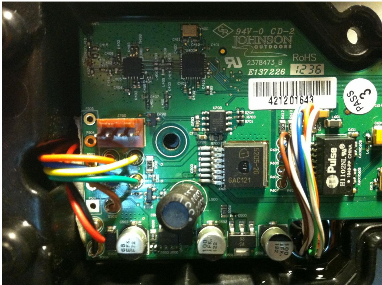
Figure 6 - RF Board detail. Antenna is short black wire in top left of photo. Approx. 1 inch long.
