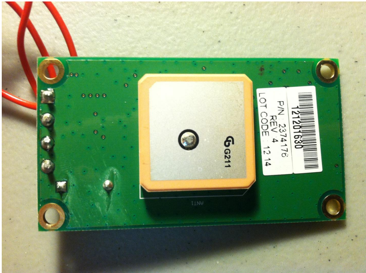
Figure 4 - Compass/combination board, bottom. GPS antenna
