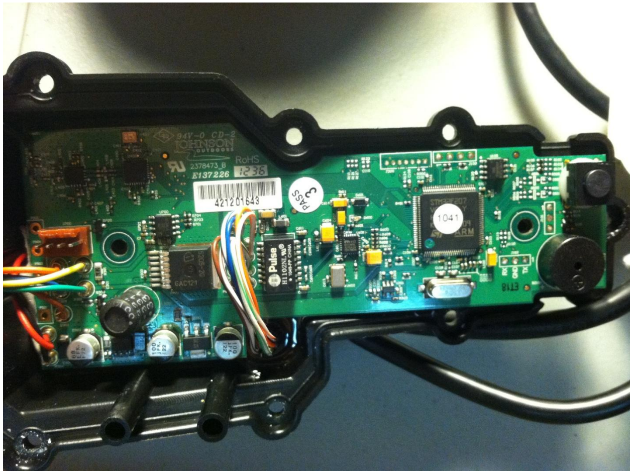
Figure 5 - RF Board
