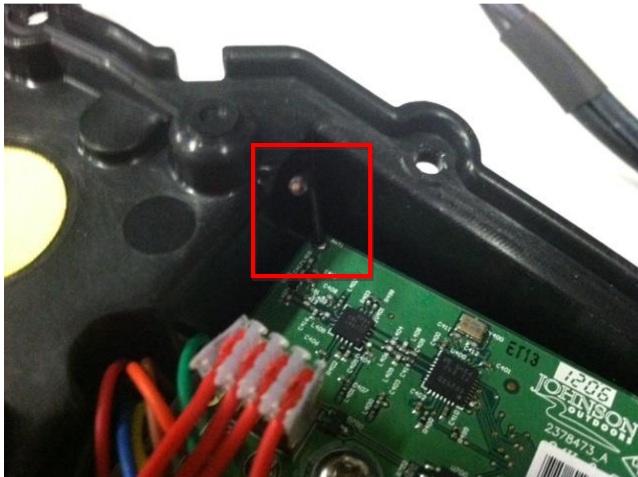
Figure 13 - Antenna, seen in red box
