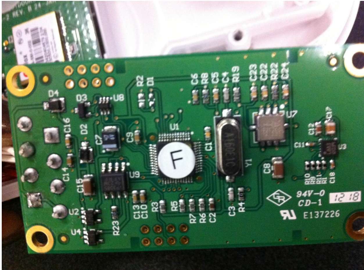
Figure 7 - Transmitter Board, Detail
