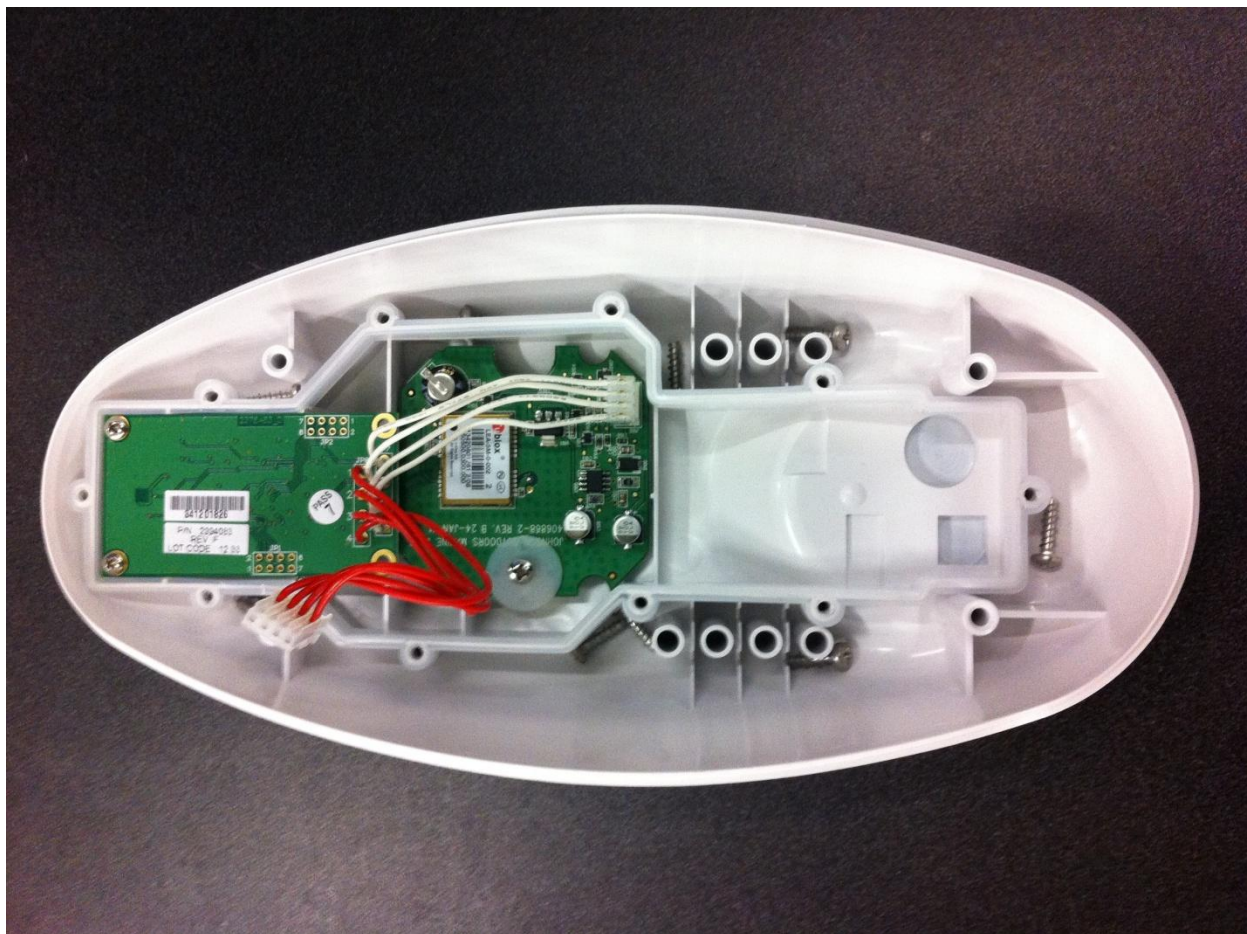
Figure 3 - Transmitter board removed
