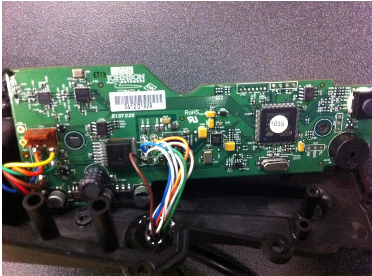
Figure 12 - Transmitter Board
