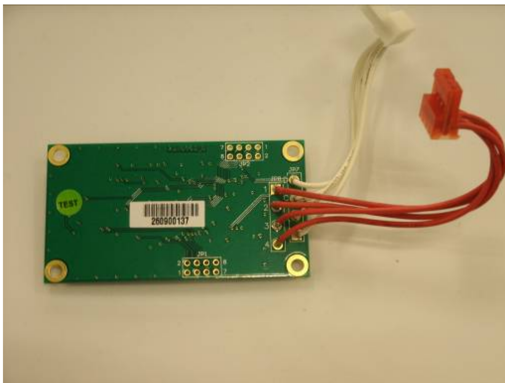
Figure 6 - i-Pilot Controller Internal, Daughter Board 2, Bottom
