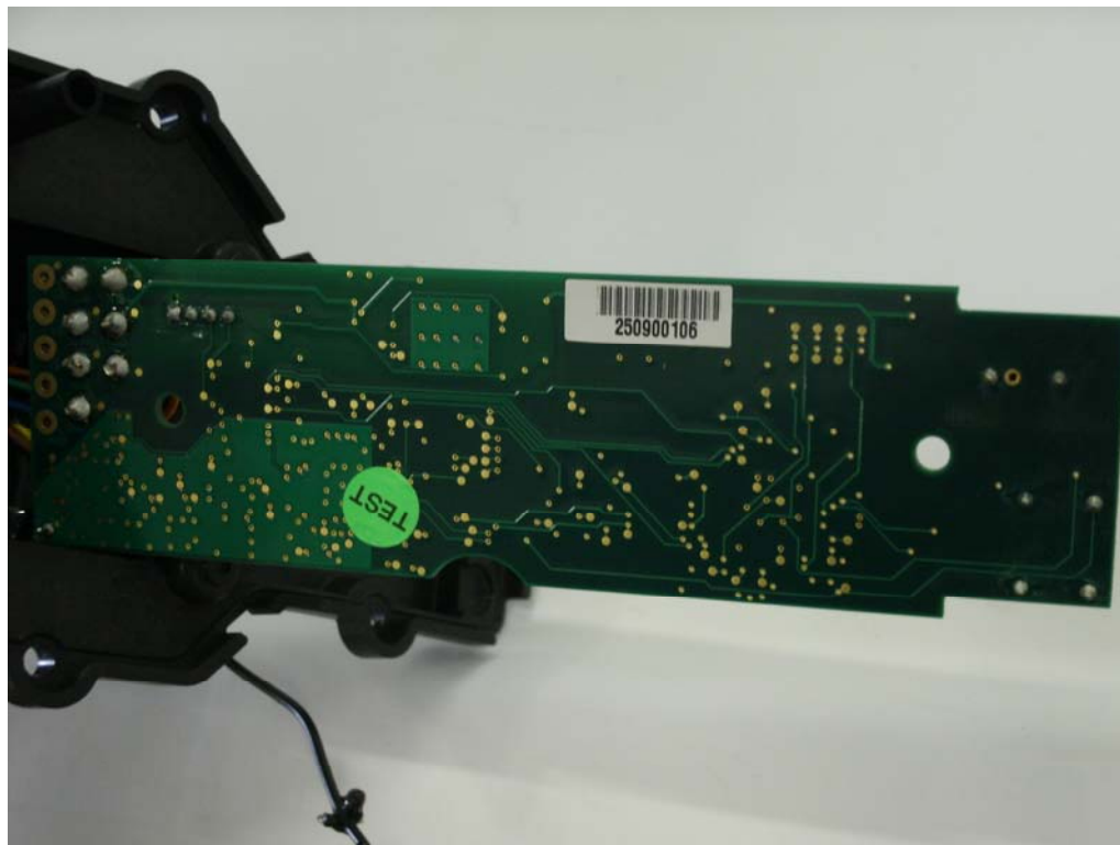
Figure 9 - i-Pilot Controller Internal, Main Board, Bottom
