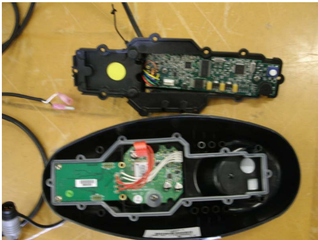
Figure 2 - i-Pilot Controller Internal, Opened
