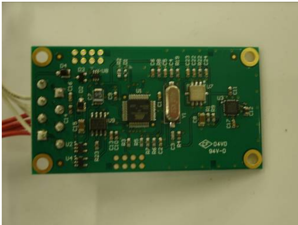
Figure 5 - i-Pilot Controller Internal, Daughter Board 2, Top
