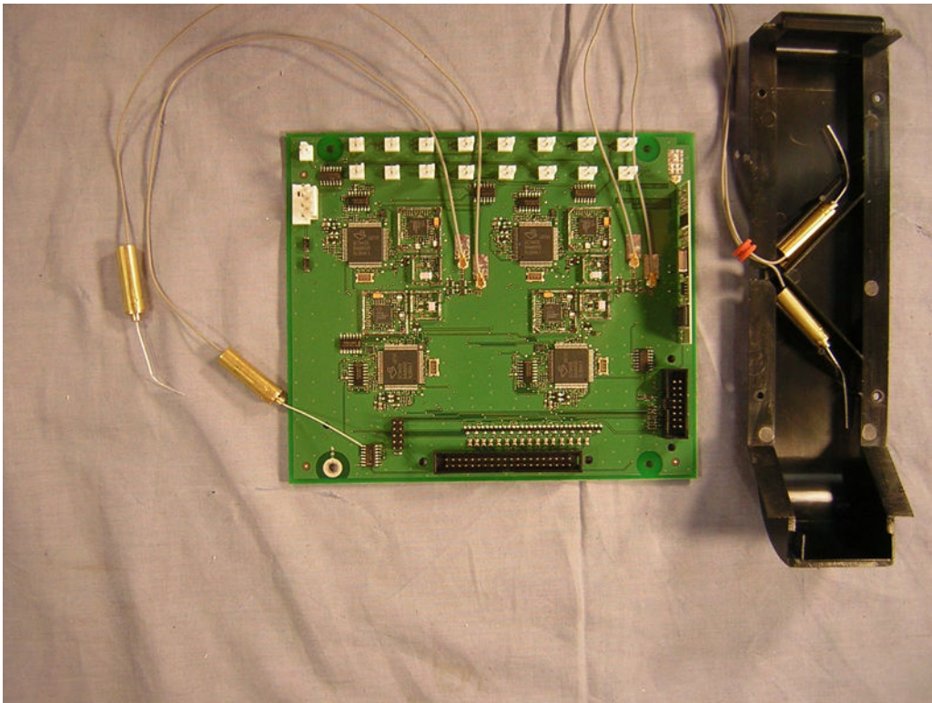
RF board w/ all four antennas connected
