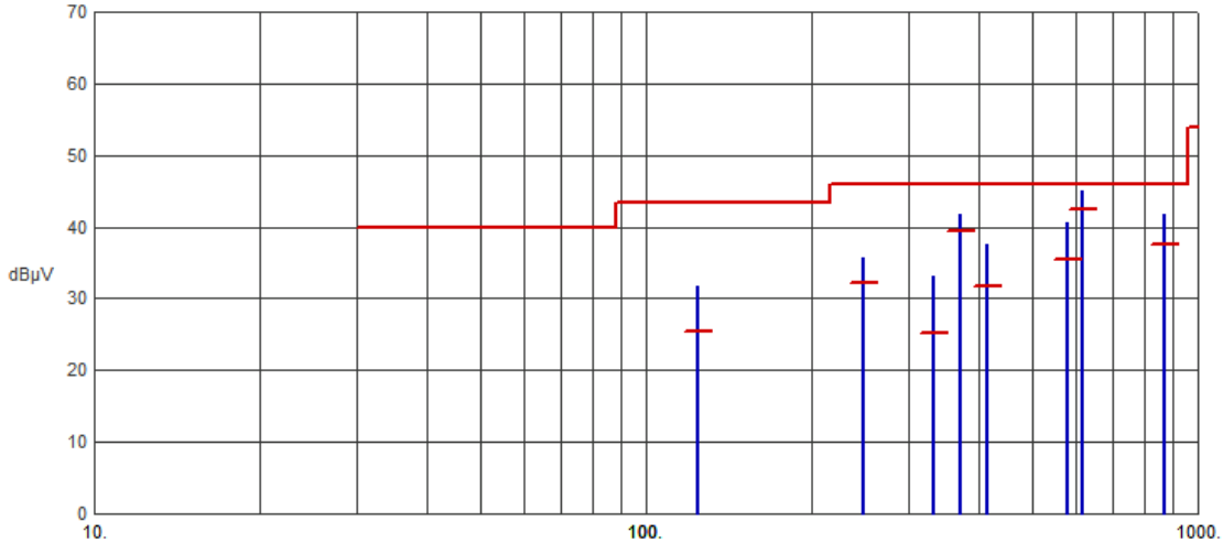
Test No.: 179.11, Radiated Emissions - Horizontal Polarity
