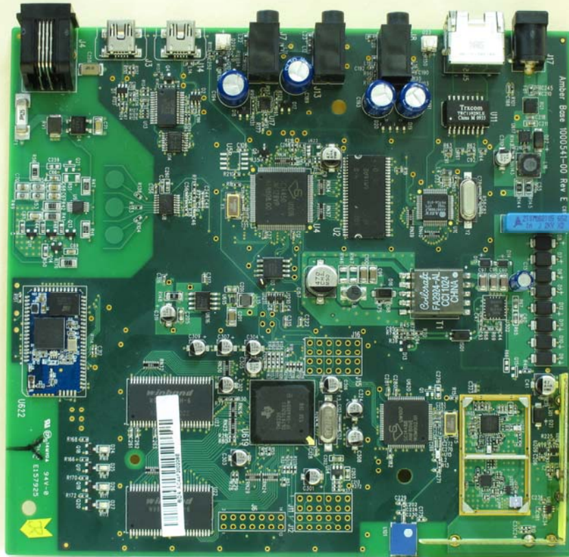
Cans removed - Component Side
