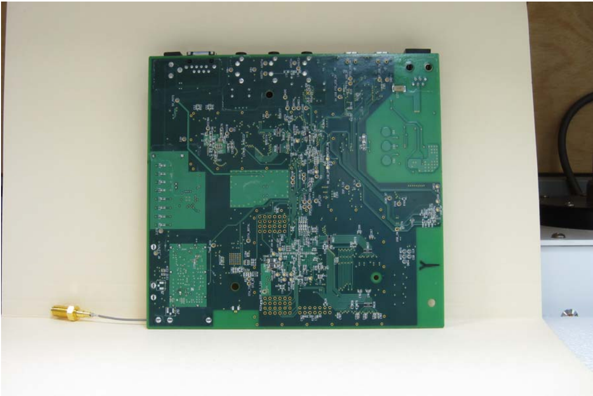
Solder Side
