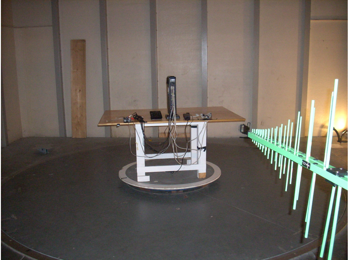
Radiated EMI (Dialer and Fusion)
