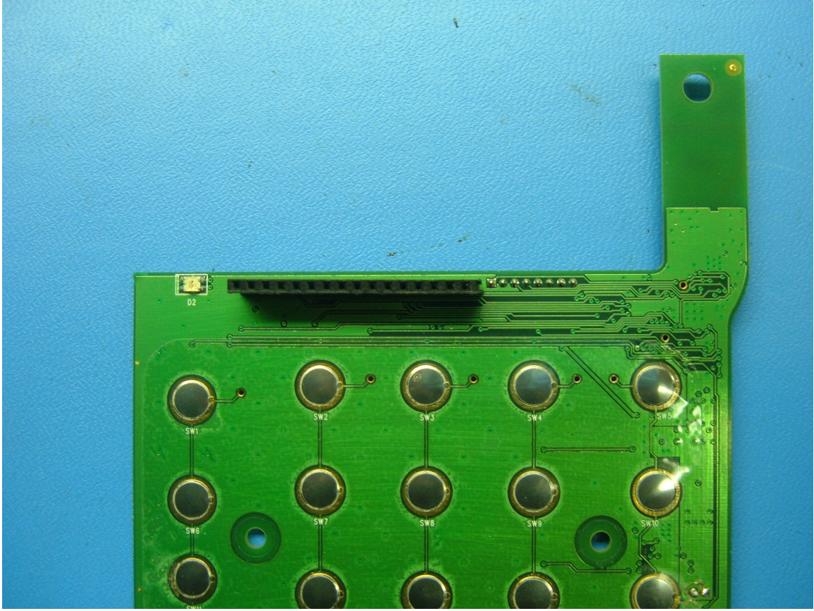
Back side of dialer RF section
