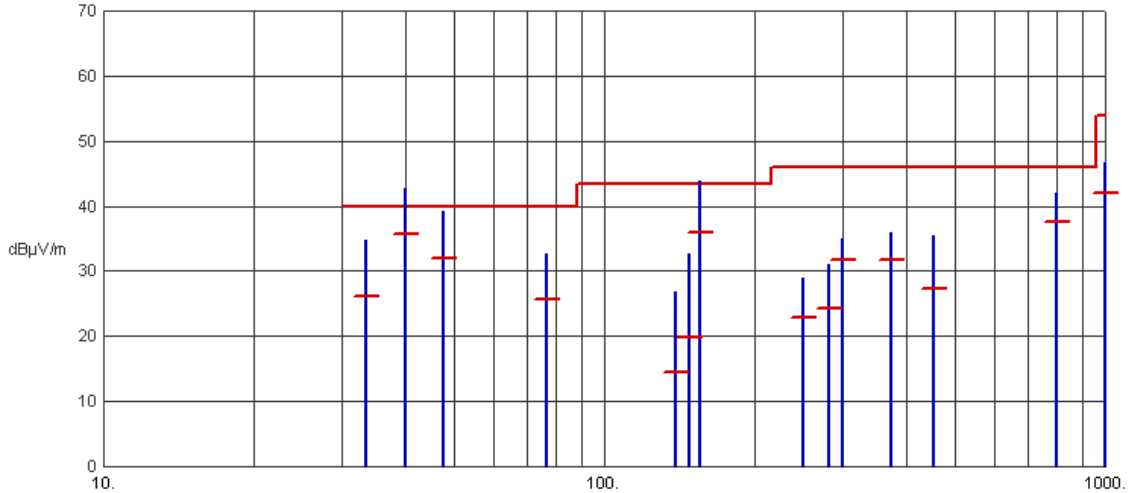
Test No.: 165-14, Radiated Emissions - Horizontal Polarity
