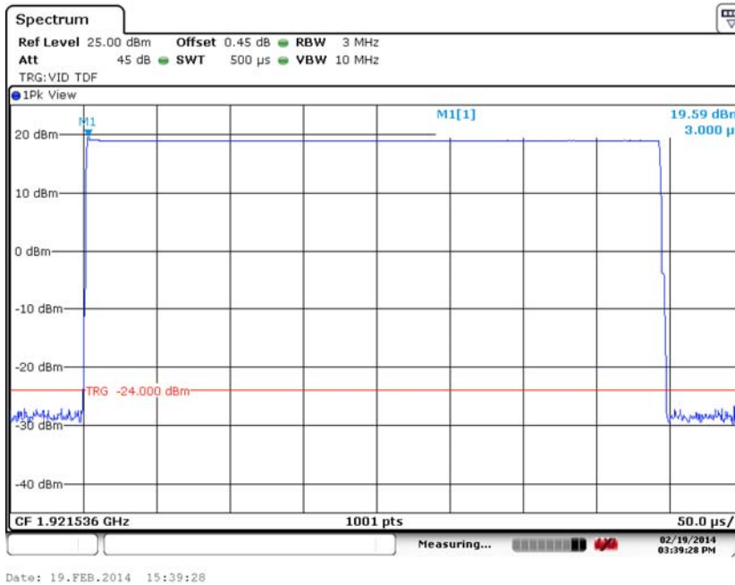
Channel 4 – BB4
