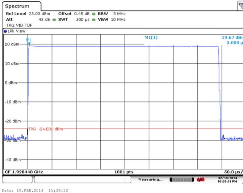
Channel 0 – BB4
