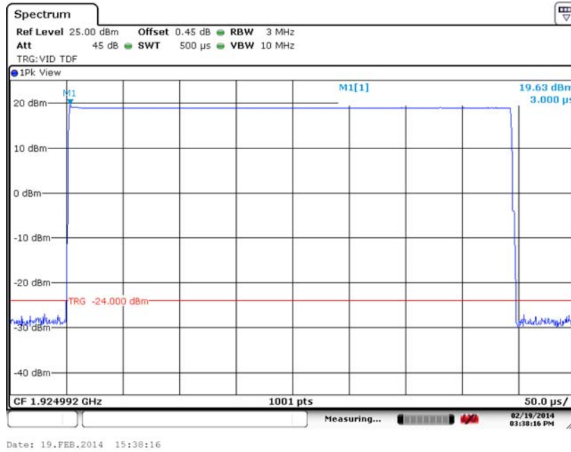
Channel 2 – BB4
