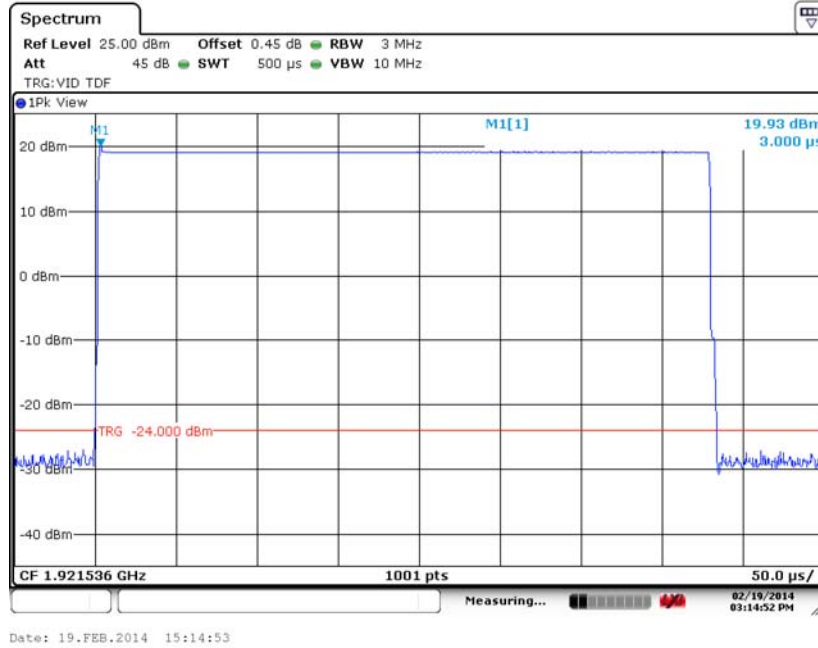
Channel 4 – BB1
