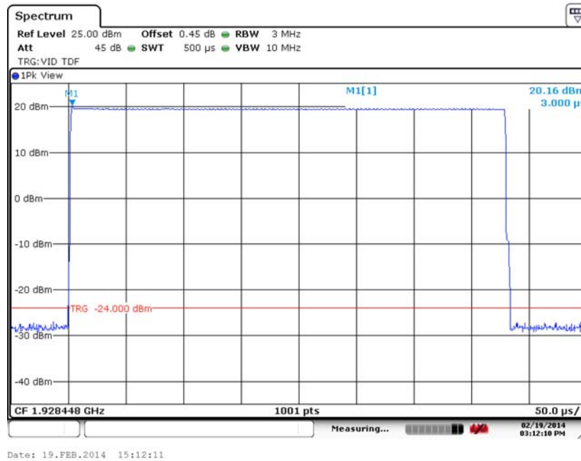
Channel 0 – BB1
