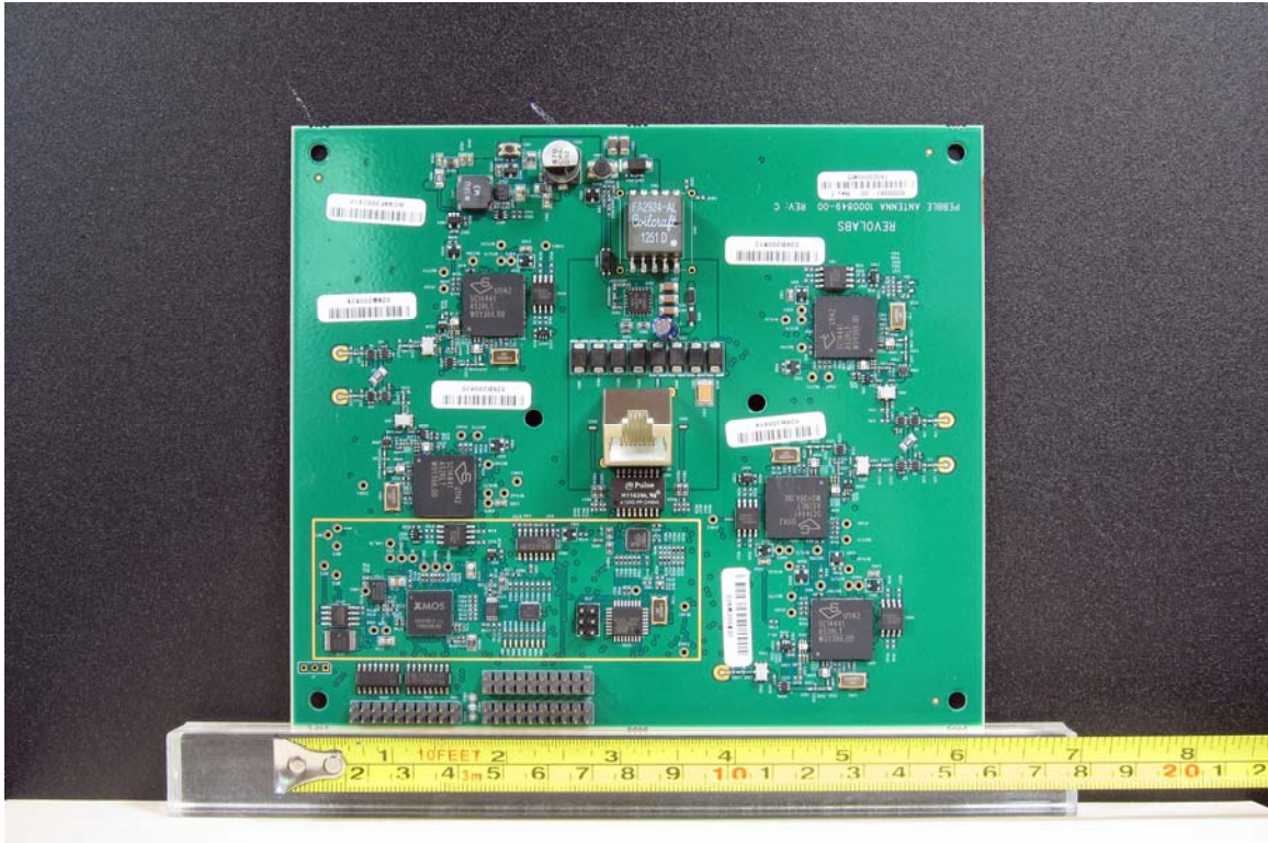
PCB Front
