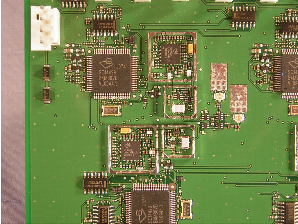
RF cans removed (8 channel version)
