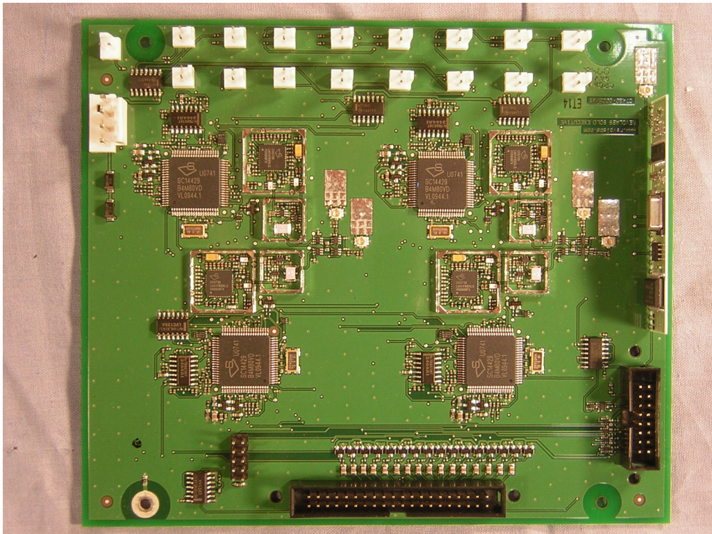
RF cans removed (8 channel version is shown, 4 channel version does not populate the 2nd half of the board )
