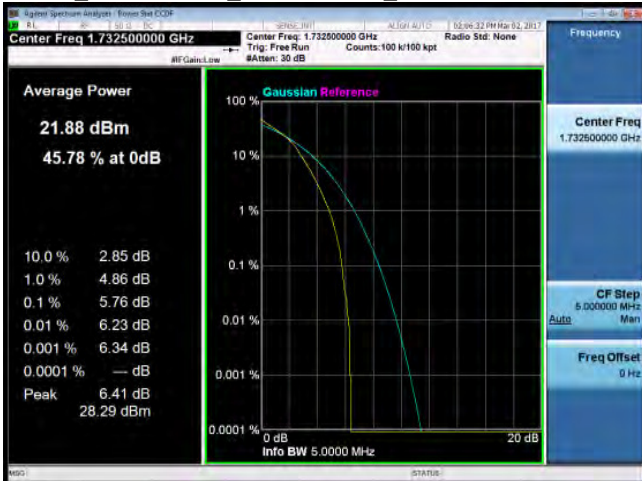
LTE_Band4 5MHz_16-QAM 25 0_MidCH20175-1732.5
