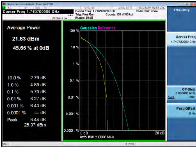
LTE_Band4 1.4MHz_16-QAM 6 0_LowCH19957-1710.7
