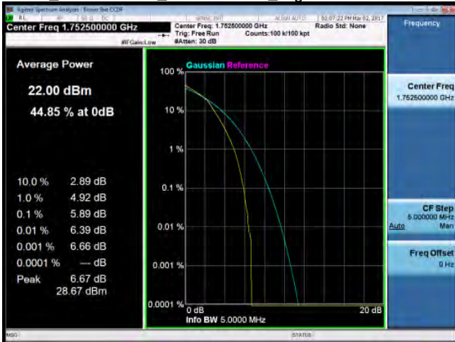
LTE_Band4 5MHz_16-QAM 25 0_HighCH20375-1752.5
