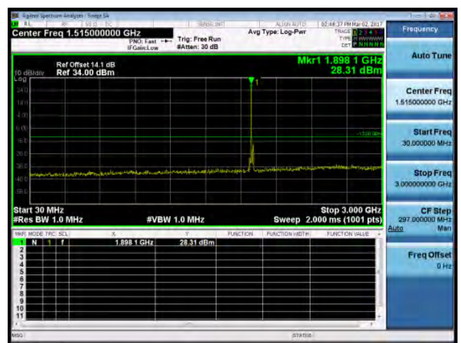
30MHz-3GHz_Band25_20MHz_QPSK_1_0_HighCH26590-1905
