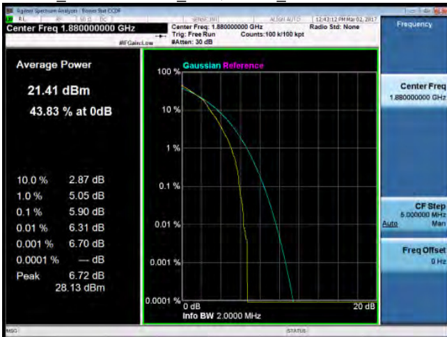
LTE_Band2 1.4MHz_16-QAM 6 0_MidCH18900-1880
