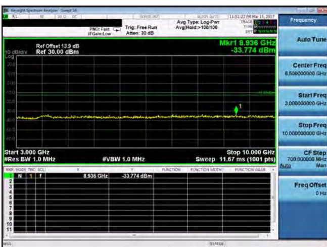
3GHz-10GHz_Band26_3MHz_QPSK_1_0_LowCH26705
