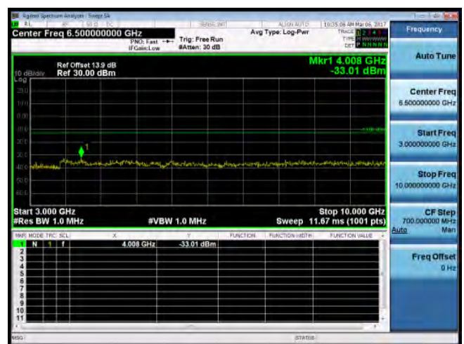
3GHz-10GHz_Band12_1.4MHz_QPSK_1_0_HighCH23173-715.3
