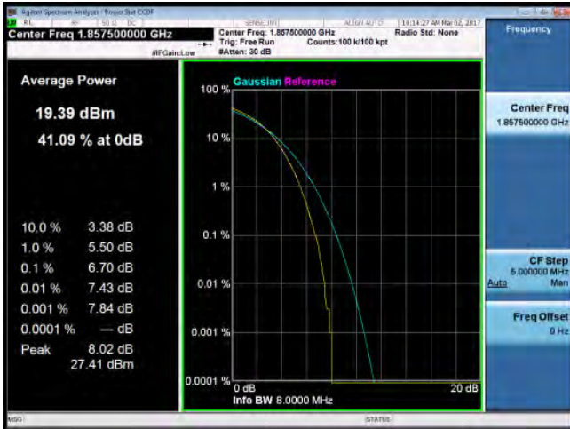
LTE_Band2 15MHz_16-QAM 75 0_LowCH18675-1857.5
