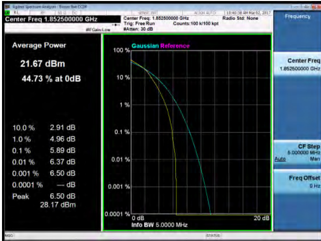
LTE_Band2 5MHz_16-QAM 25 0_LowCH18625-1852.5
