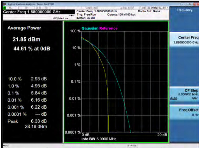
LTE_Band2 5MHz_16-QAM 25 0_MidCH18900-1880
