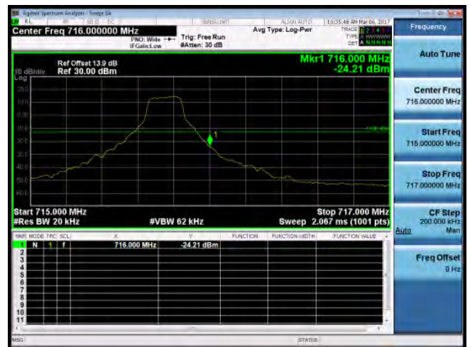
Band Edge_Band12_1.4MHz_QPSK_1_5_HighCH23173-715.3
