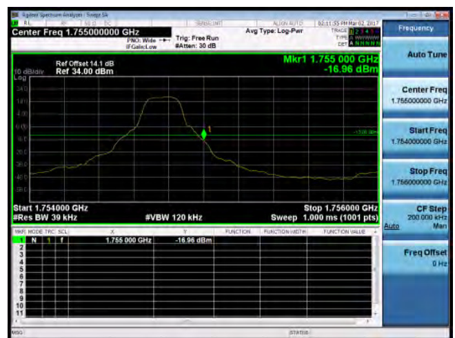
Band Edge_Band4_3MHz_QPSK_1_14_HighCH20385-1753.5
