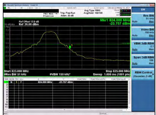
Band Edge_Band26_5MHz_QPSK_1_24_HighCH26765
