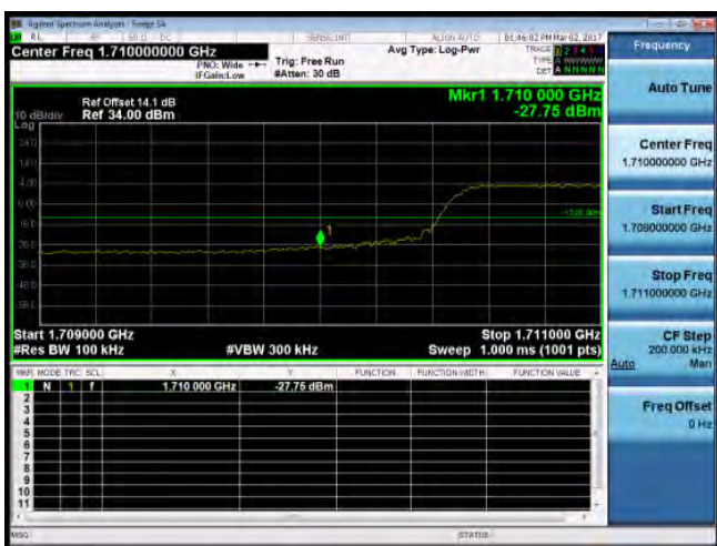
Band Edge_Band4_10MHz_QPSK_50_0_LowCH20000-1715
