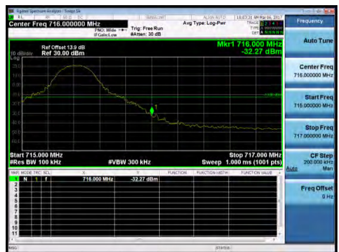
Band Edge_Band12_10MHz_QPSK_1_49_HighCH23130-711
