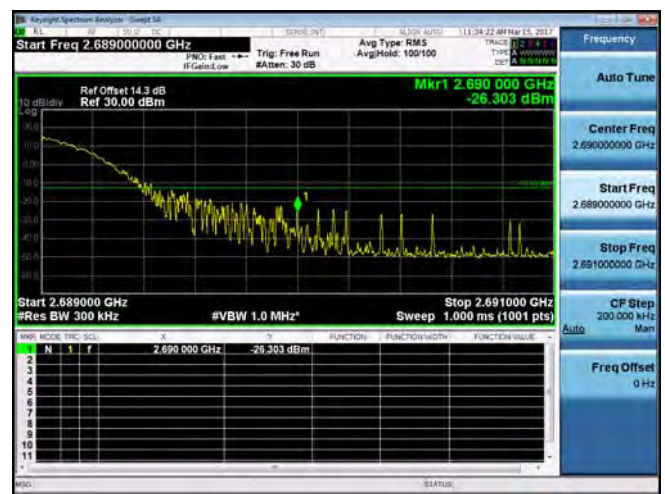
Band Edge_Band41_20MHz_QPSK_1_99_HighCH41490
