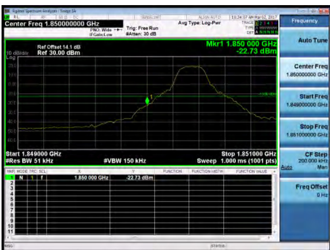
Band Edge_Band2_5MHz_QPSK_1_0_LowCH18625-1852.5
