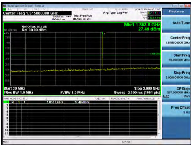
30MHz-3GHz_Band2_5MHz_QPSK_1_0_MidCH18900-1880
