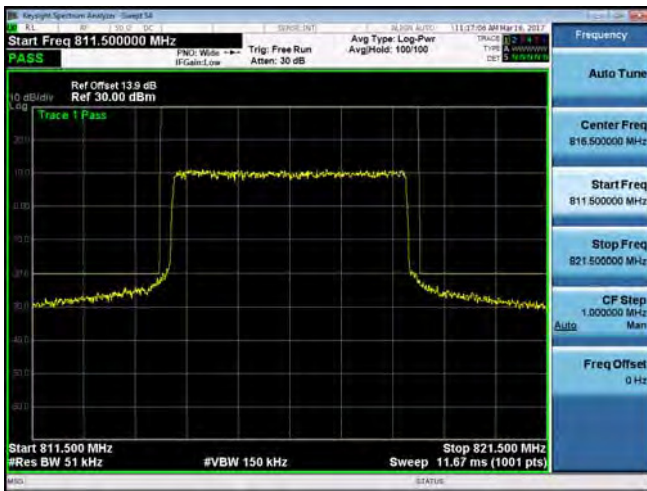
Emission Mask_Band26 for Part 90S_5M_QPSK_MID_RB25,0
