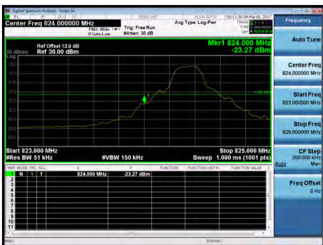
Band Edge_Band5_5MHz_QPSK_1_0_LowCH20425-826.5
