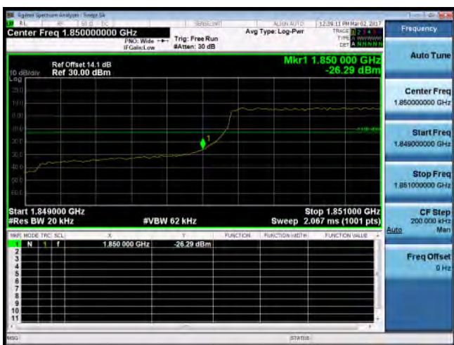
Band Edge_Band2_1.4MHz_QPSK_6_0_LowCH18607-1850.7
