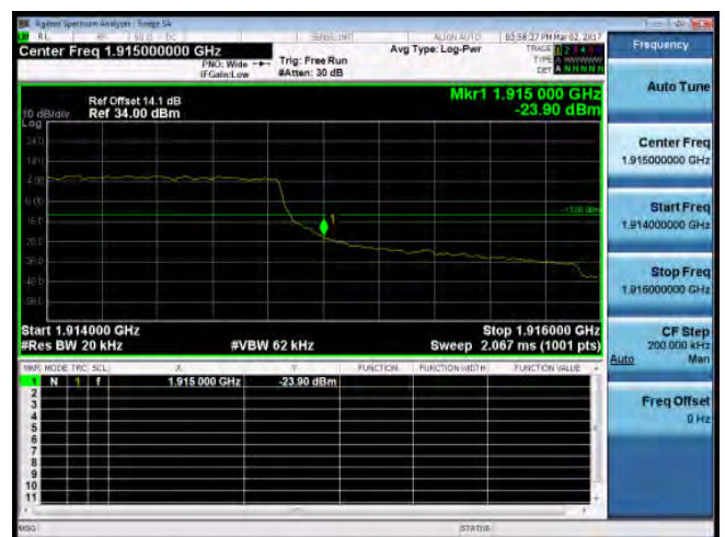
Band Edge_Band25_1.4MHz_QPSK_6_0_HighCH26683-1914.3
