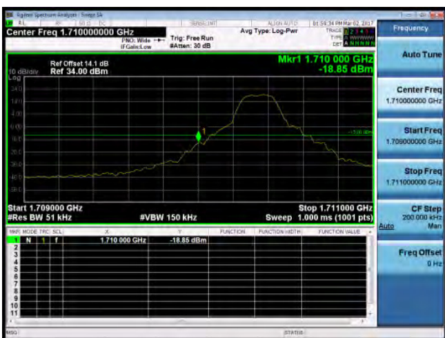
Band Edge_Band4_5MHz_QPSK_1_0_LowCH19975-1712.5
